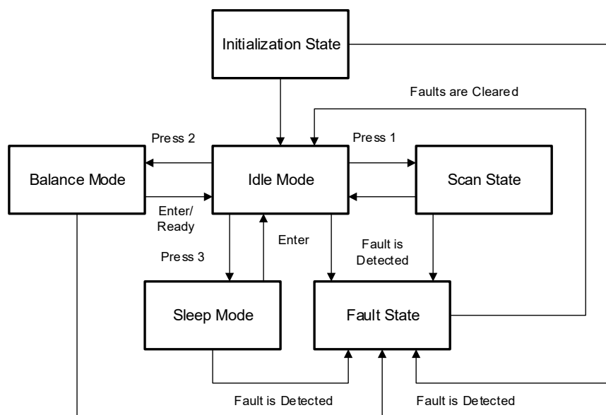
Figure 1. Sample Code State Machine Flow Diagram
