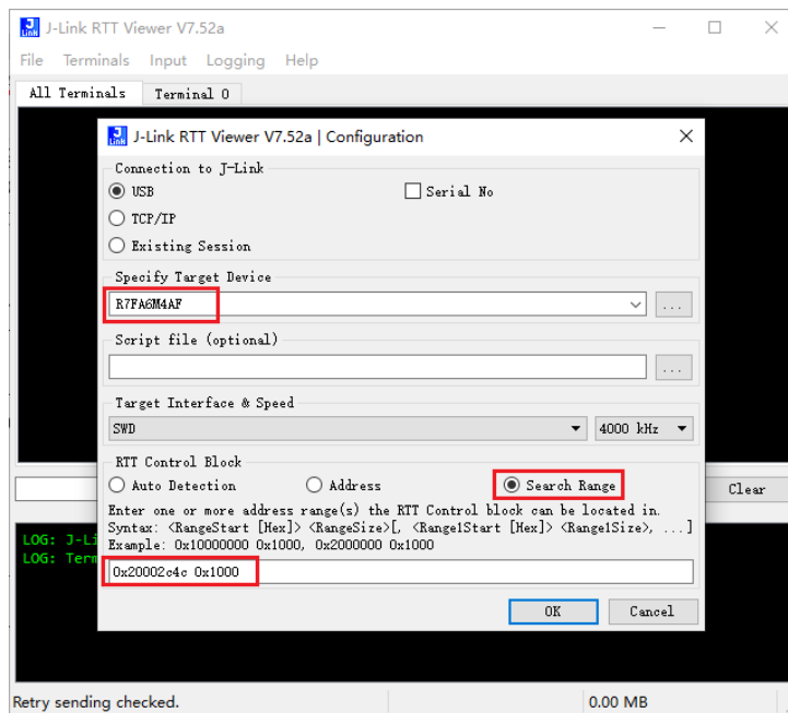
Figure 4. J-Link RTT Viewer
