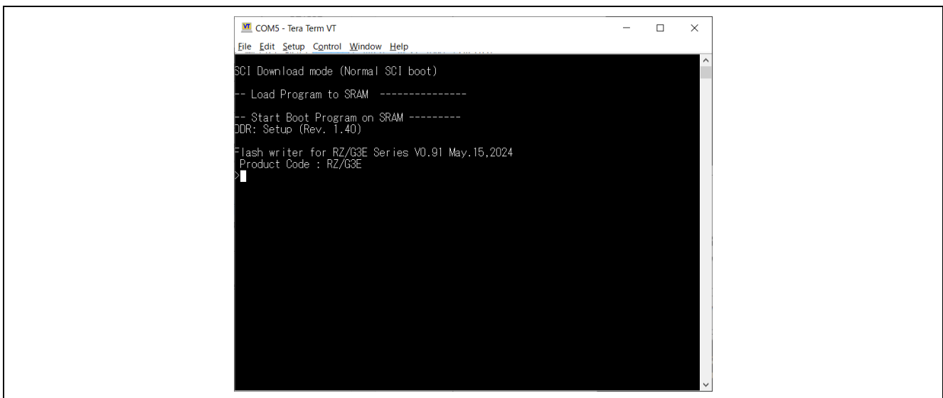
Figure 5-5. Flash Writer invocation
