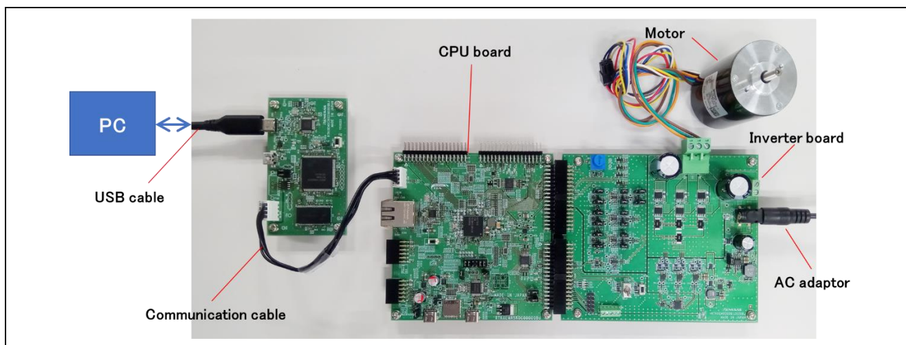
Figure 6-1 Hardware Configuration
