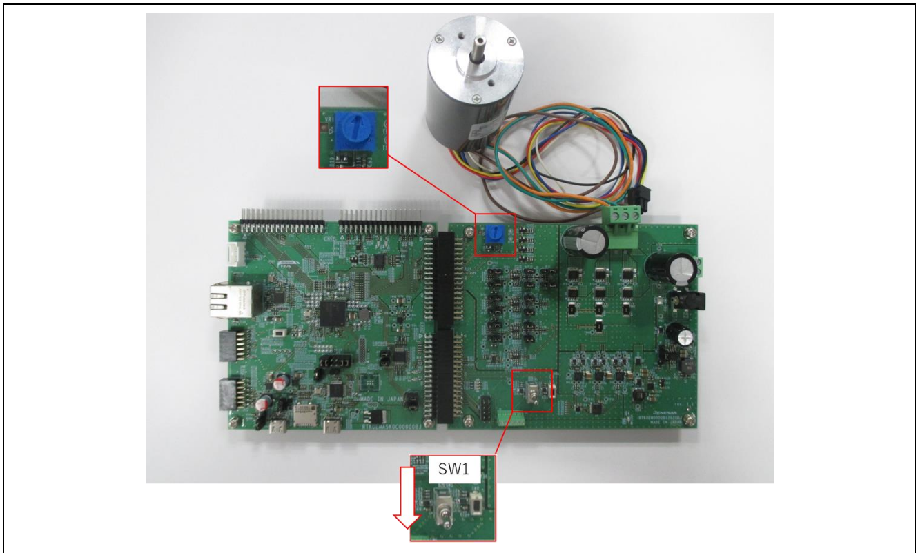
Figure 4-4 Hardware configuration
