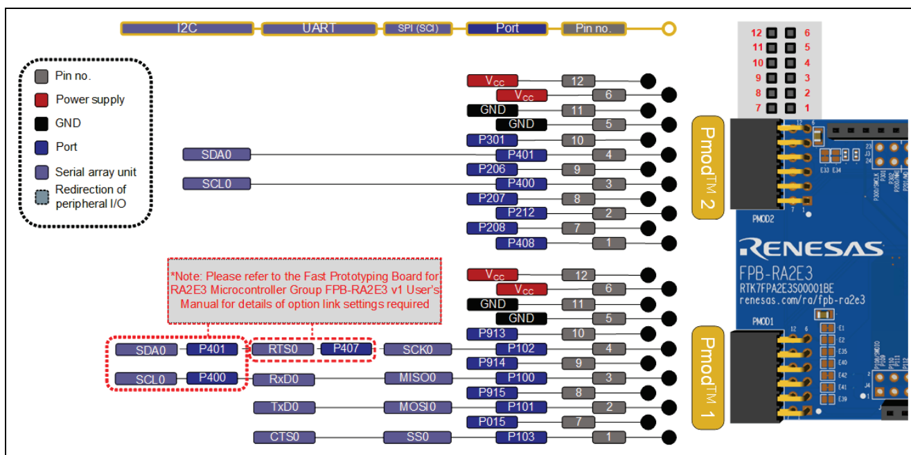
Figure 3. FPB-RA2E3 Pmod Interface
