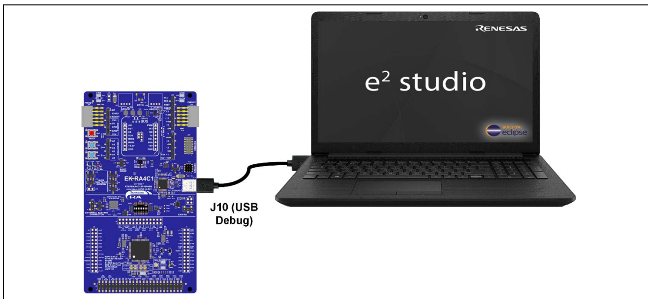
Figure 32. Connecting the EK-RA4C1 Board to the Host PC via USB Debug Port
