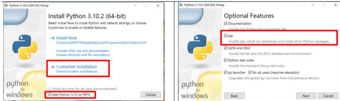
Figure 5-1 Installing Python
