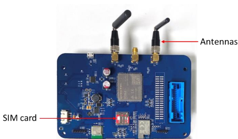
Figure 4-9 SIM card and Antennas
