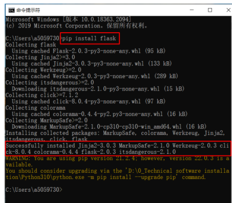
Figure 5-2 Installing flask
