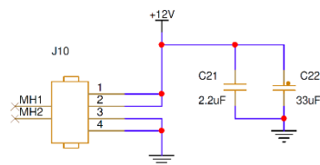
Figure 4-2 Power connector J10
