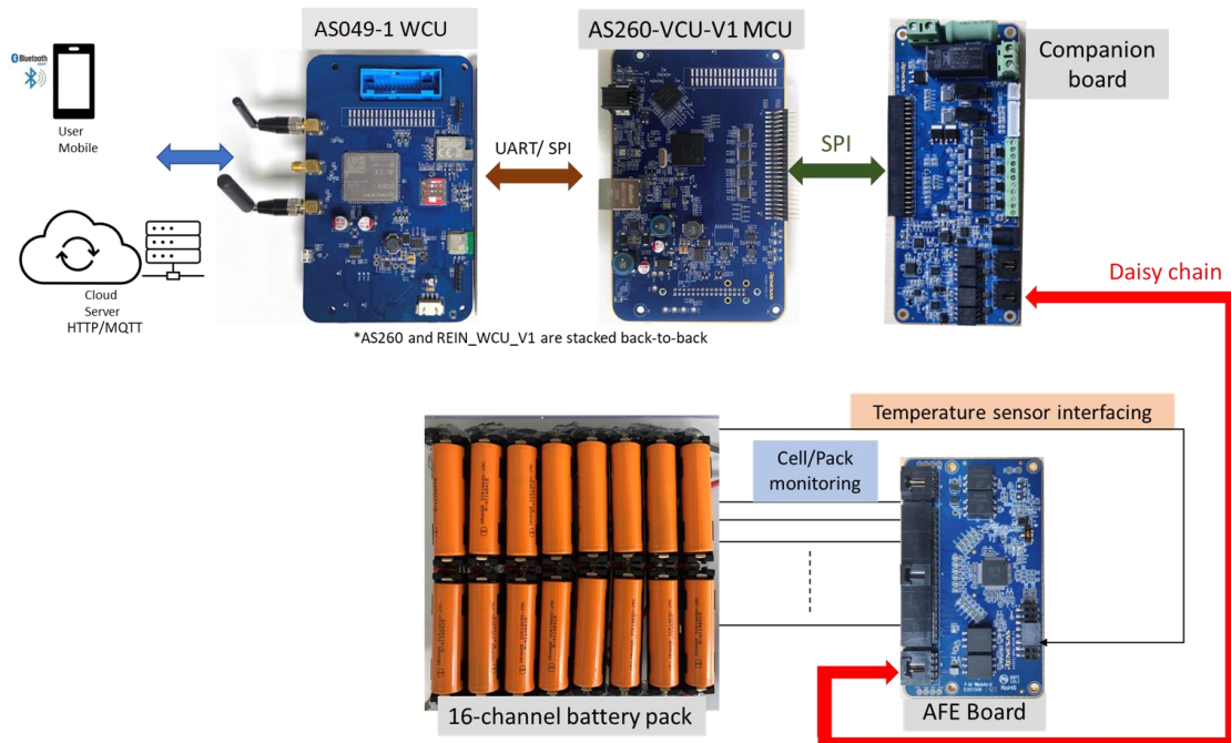
Figure 5-6 System Connection flow
