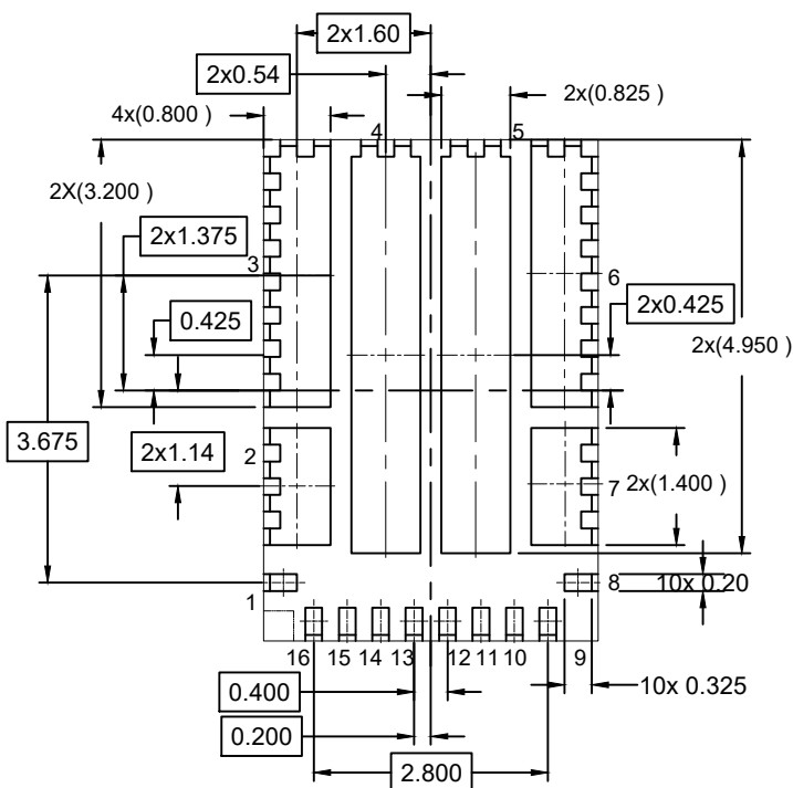
Bottom View
