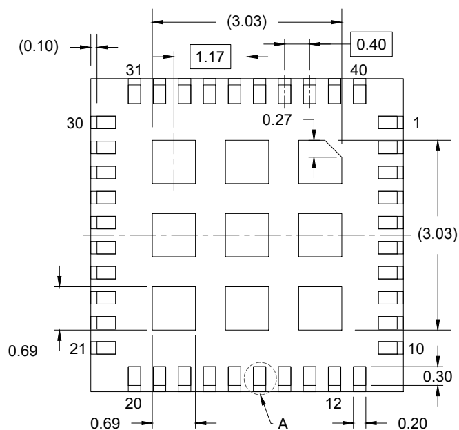
BOTTOM VIEW
