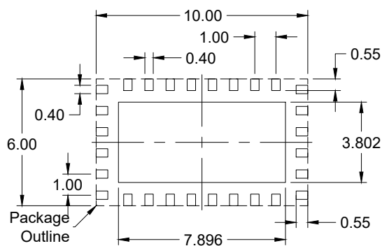
RECOMMENDED LAND PATTERN (PCB Top View)
