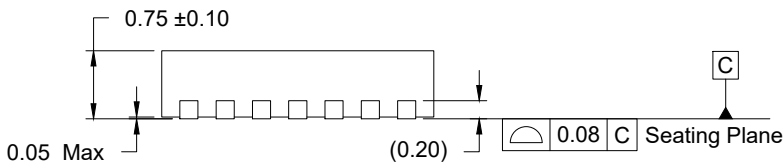
SIDE VIEW
