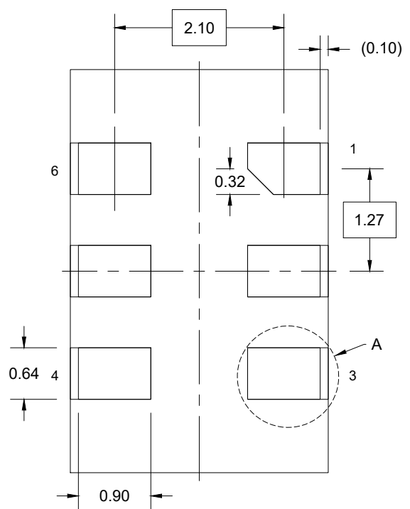
BOTTOM VIEW
