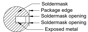
Detail A
