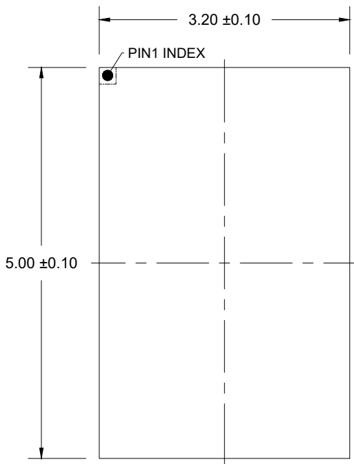
TOP VIEW
