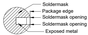
Detail A
