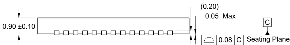
SIDE VIEW
