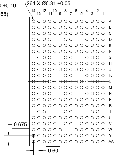
BOTTOM VIEW
