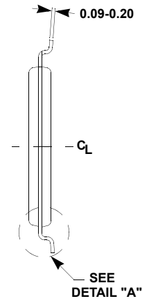
BOTTOM VIEW
