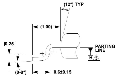
DETAIL "A" SCALE: (NONE) (VIEW ROTATED 90° C.W.)
