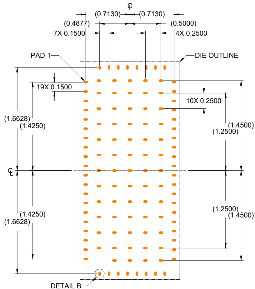
RECOMMENDED LAND PATTERN (Substrate Top View)
