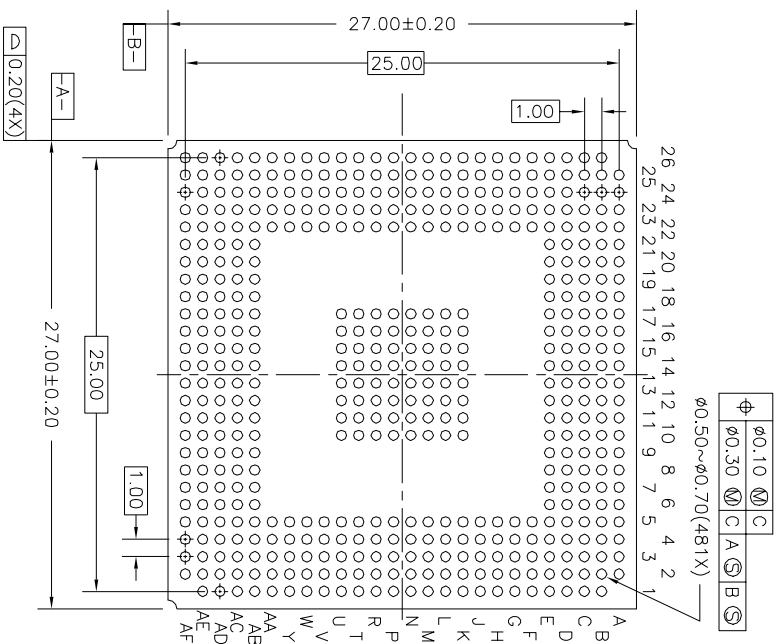
BOTTOM VIEW (BALL SIDE)
