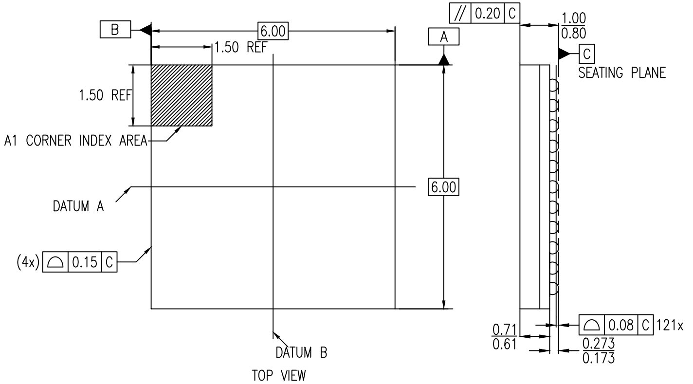
SIDE VIEW
