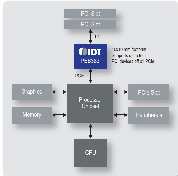
Figure 1 Motherboard Application
