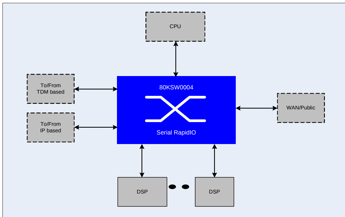
Figure 1 Application Overview
