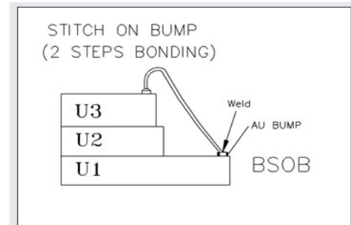
Diagram showed three stack dies from side view
