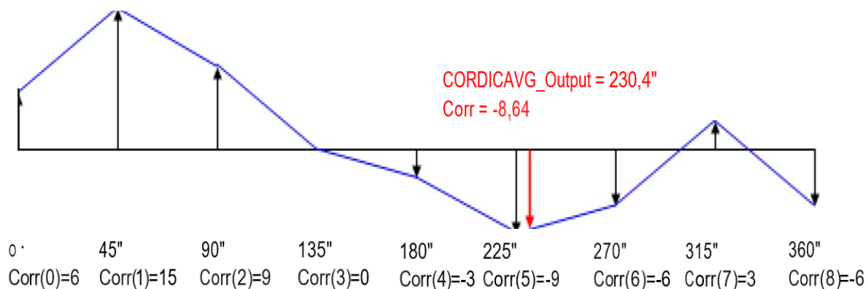
Figure 4. Linear Error Correction Example
