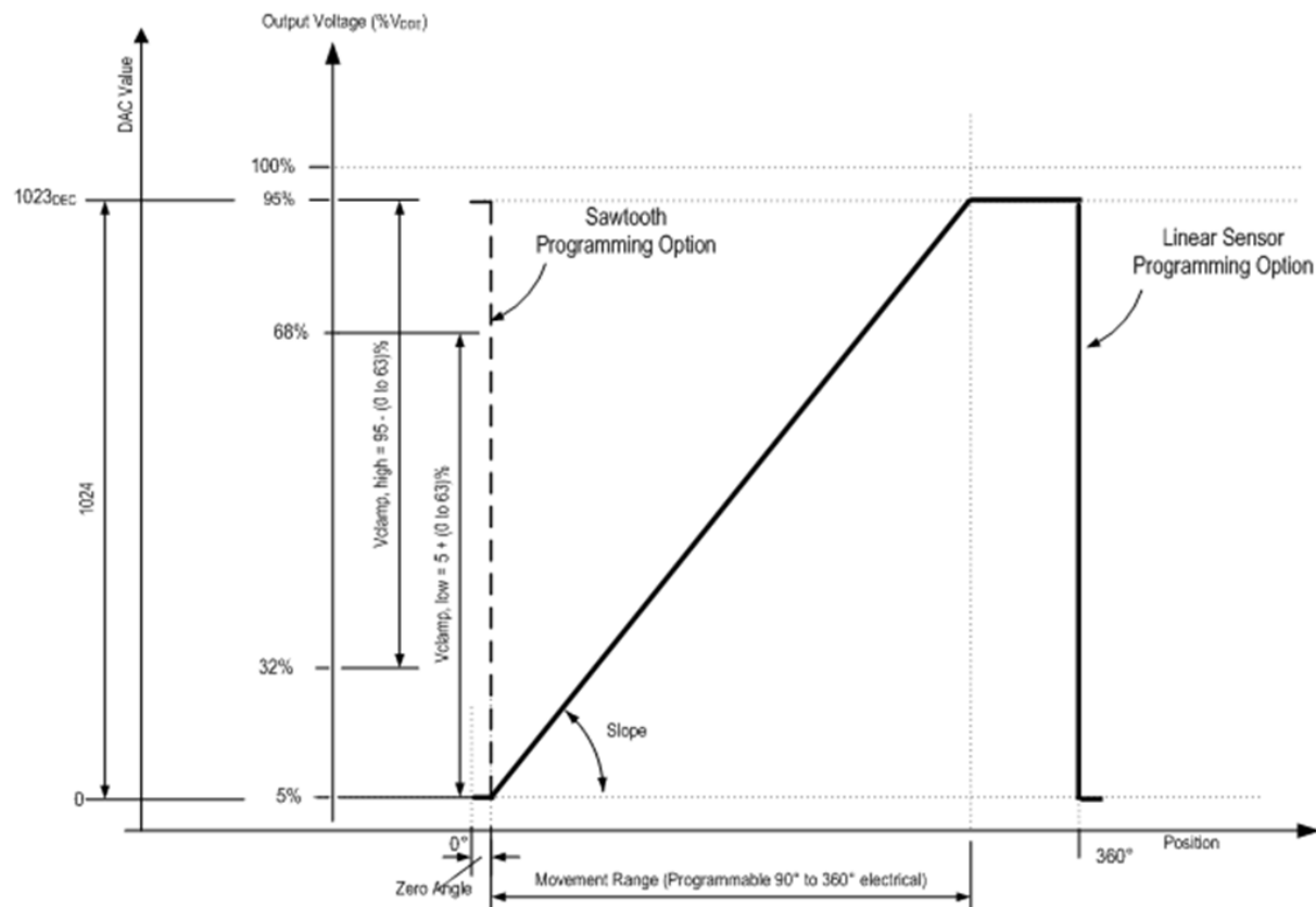
Figure 3. Clamping Example
