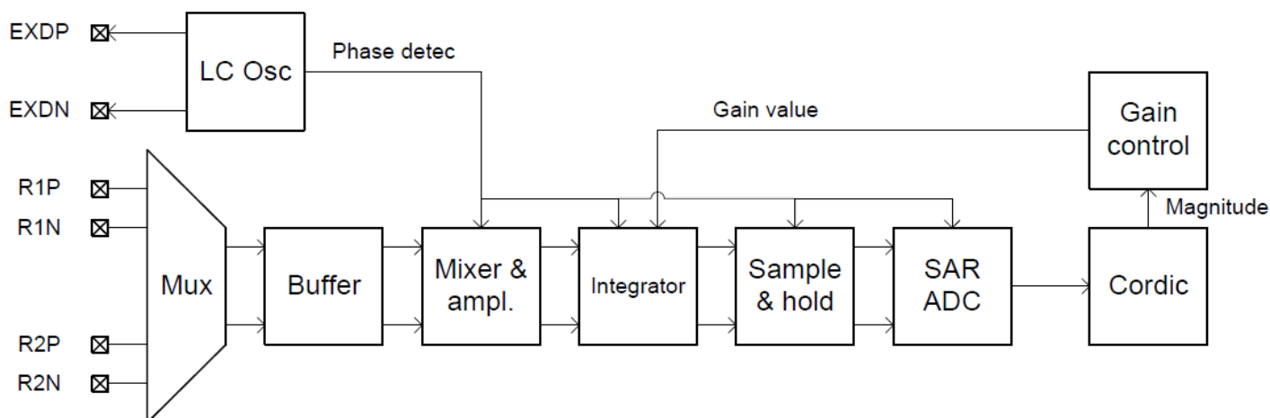
Figure 11. Gain Control
