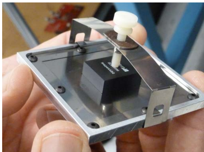
FIGURE 16. ALIGN STENCIL ONTO REPLACEMENT MODULE
