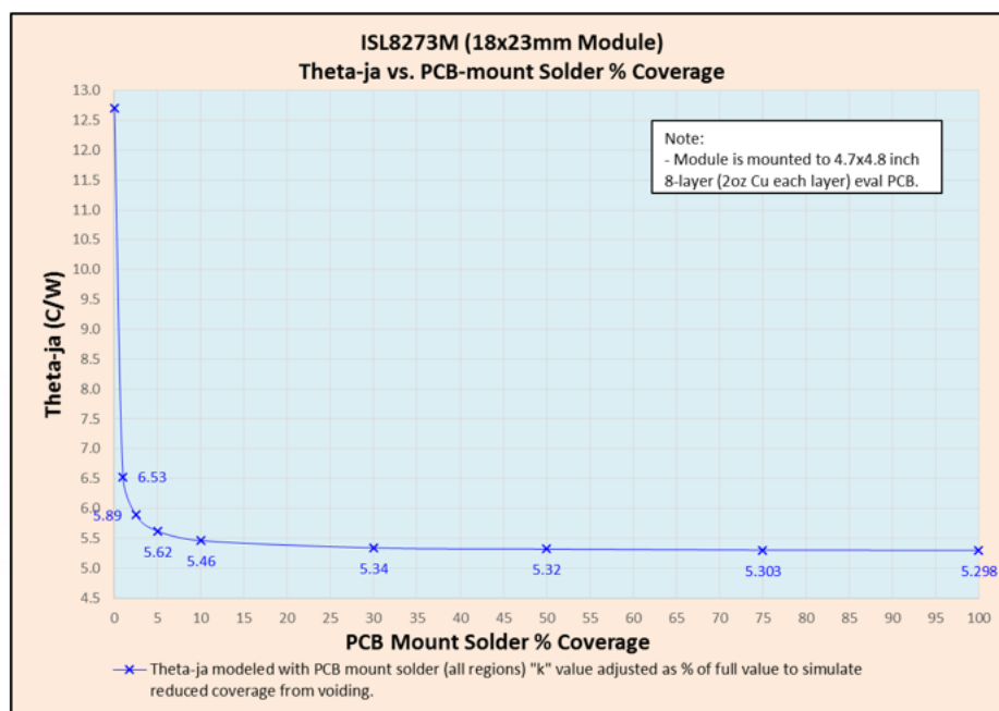
FIGURE 7. \theta_{JA} vs PCB-MOUNT SOLDER % COVERAGE
