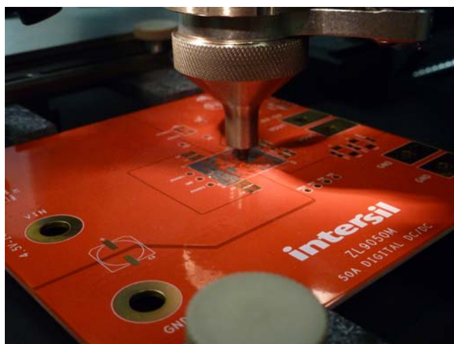
FIGURE 13. SITE REDRESS
