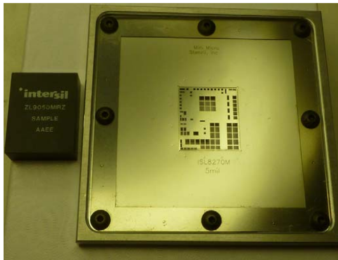
FIGURE 15. MINIATURE STENCIL
