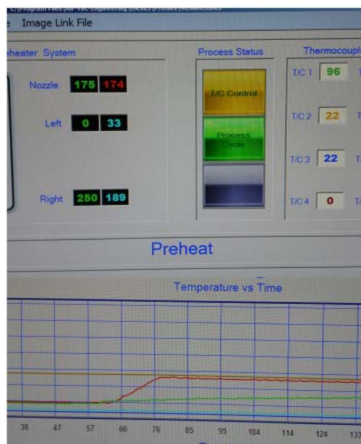
FIGURE 10. PREHEAT CONTROL
