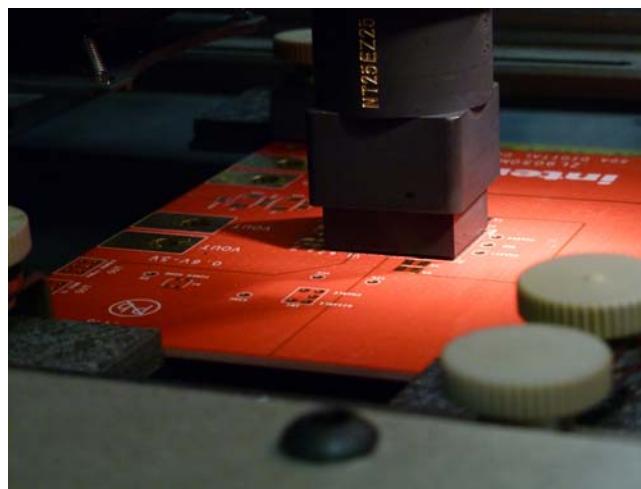
FIGURE 20. COMPONENT PLACEMENT
