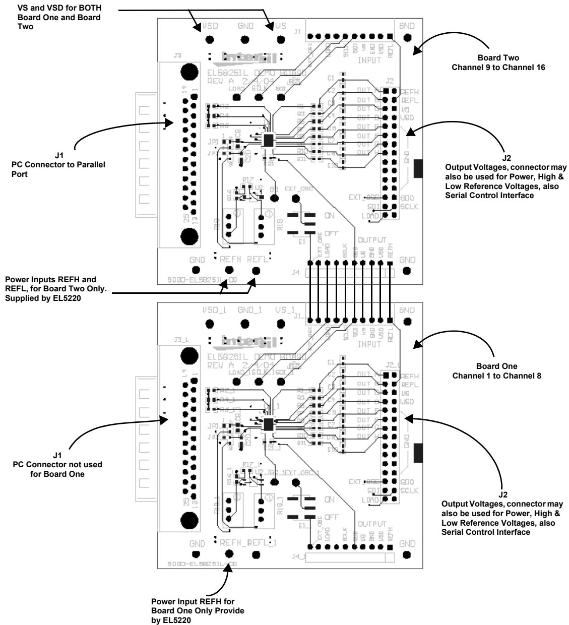
FIGURE 2. 16-CHANNEL
