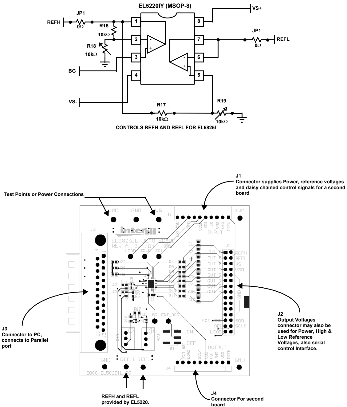
FIGURE 1. 8-CHANNEL
