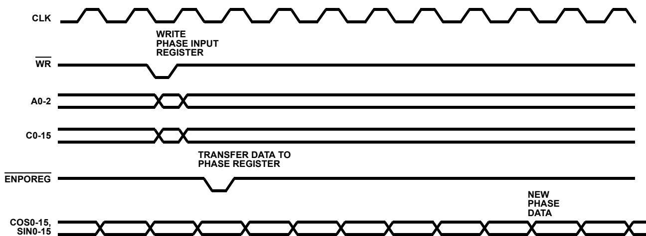
FIGURE 2. PHASE TO OUTPUT DELAY
