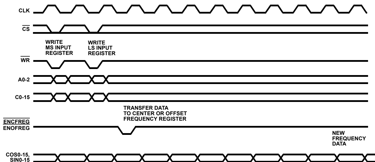
FIGURE 1. FREQUENCY TO OUTPUT DELAY
