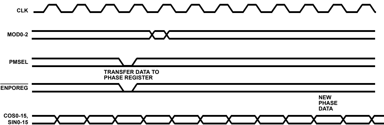
FIGURE 3. PHASE MODULATION TO OUTPUT DELAY
