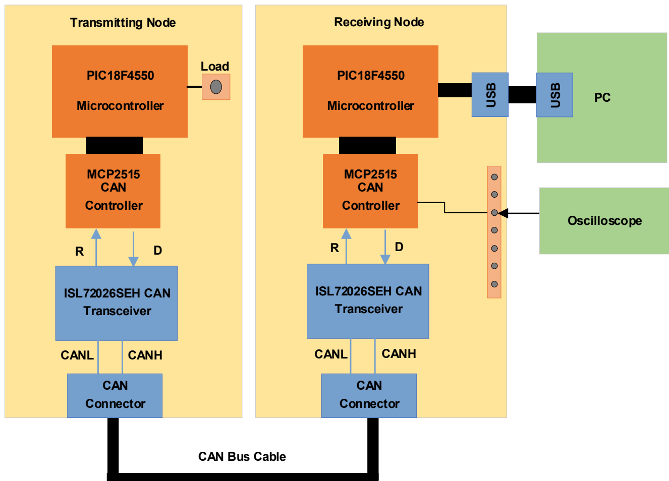
Figure 1. SEE Two Node CAN Bus System Block Diagram
