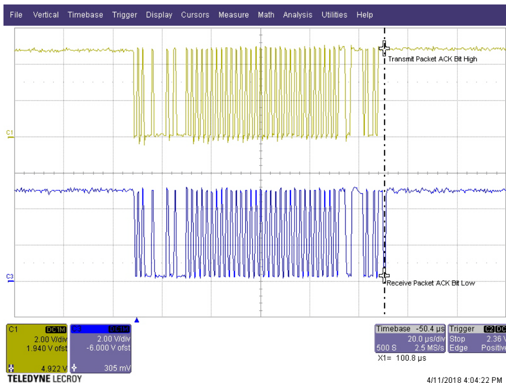
Figure 3. Scope Plot of the System CAN Data Packet
