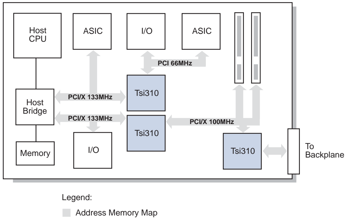
Figure 1: Host or Embedded Board Bridge Uses — Flat Address Map
