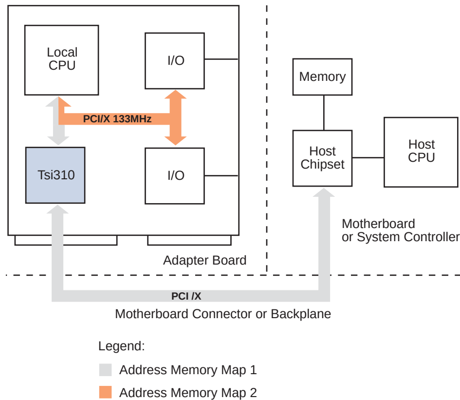
Figure 4: PCI/X Intelligent Adapter with Opaque Bridge — Shared and Independent Memory Map
