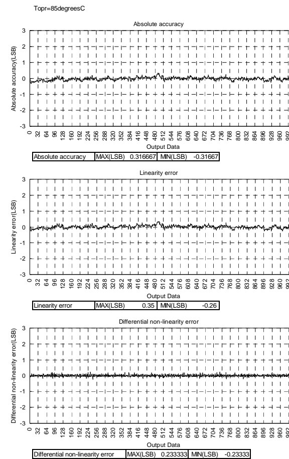
Figure35. Topr=85(degrees C)
