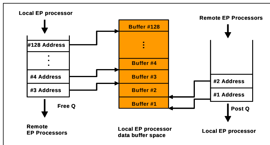
Figure 9 Inbound Queue and Data Buffer Usage
