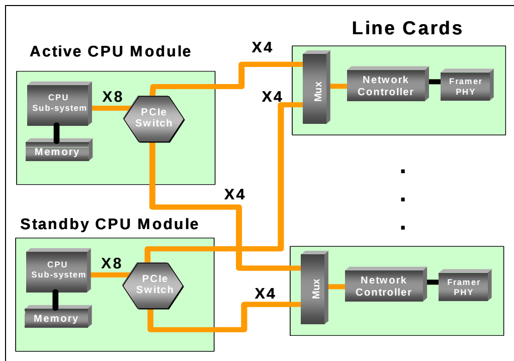
Figure 5 Dual-star Topology
