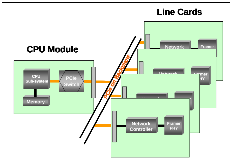
Figure 2 System Diagram of a PCIe Based Router
