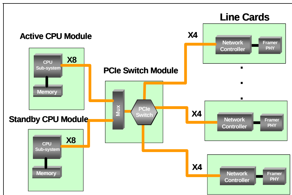
Figure 4 Dual-CPU Topology
