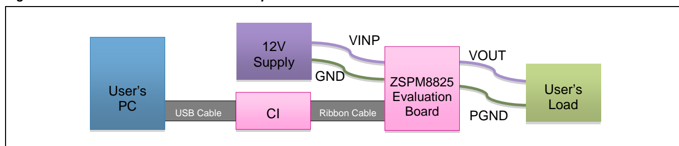
Figure 2.3 Pink Power Evaluation Kit Setup
