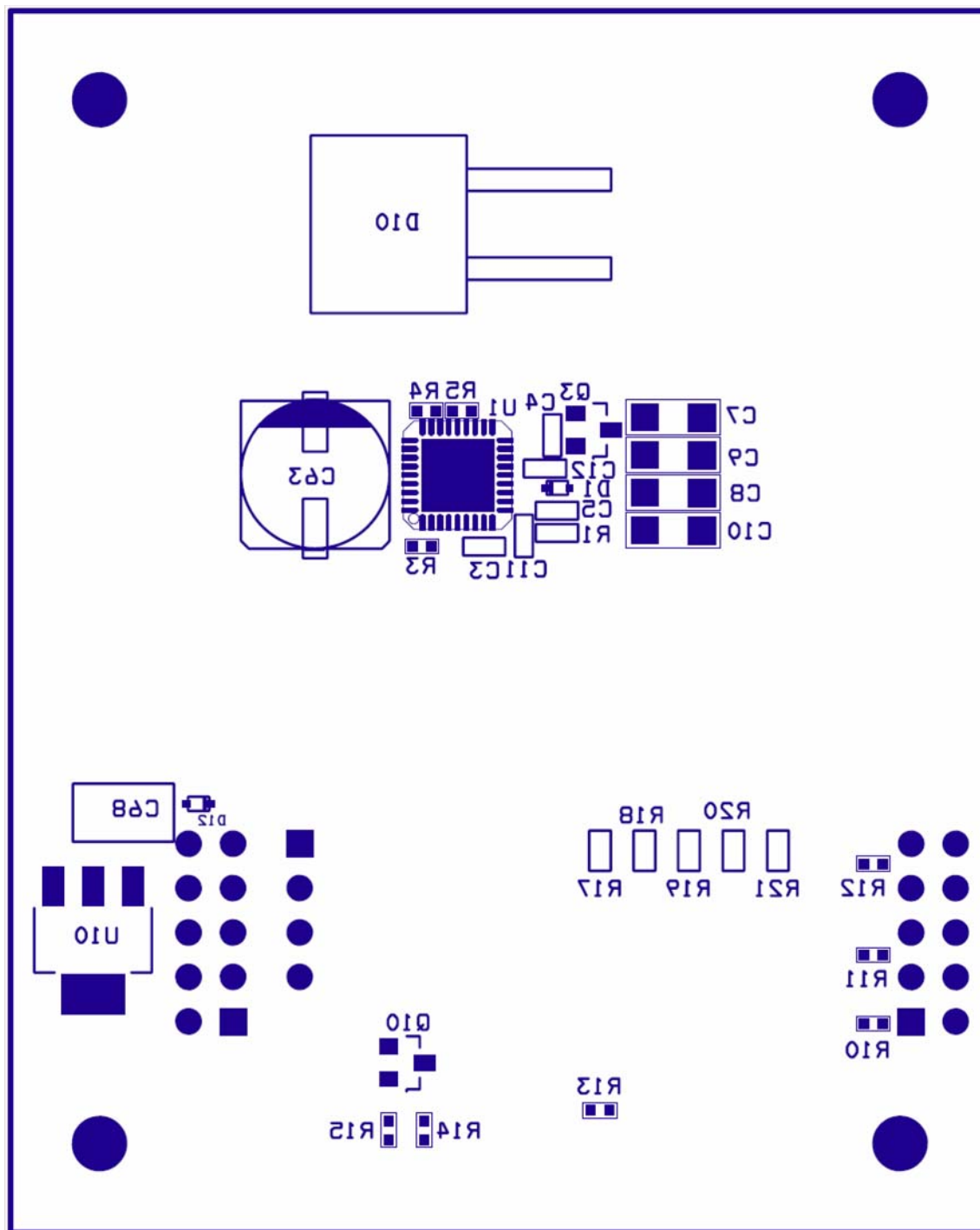
FIGURE 10. FG ZL2005PEVK4 SILK SCREEN BOTTOM (TOP VIEW - REVERSED)
