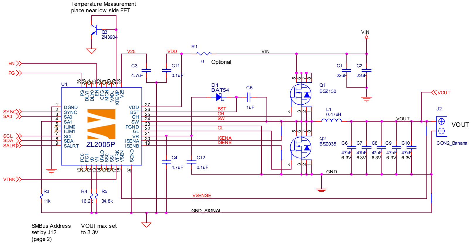
FIGURE 3. FG ZL2005PEVK4 CIRCUIT
