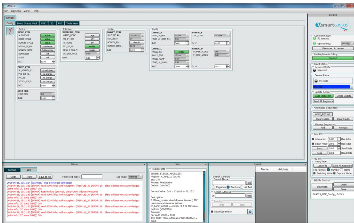
Figure 11: Main Interface
