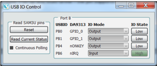
Figure 26: USB IO Control
