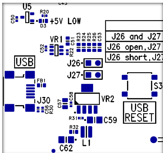
Figure 4: USB Interface Connector and Reset Switch
