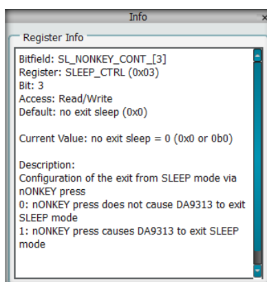
Figure 23: Info
