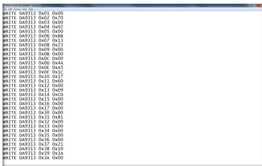
Figure 29: Register Dump (.txt File) Example
