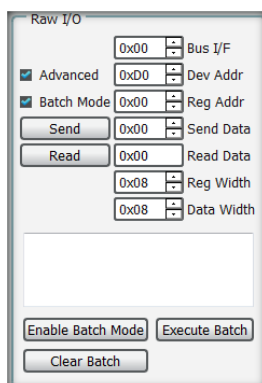
Figure 16: Raw I/O
