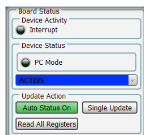
Figure 15: Board Status
