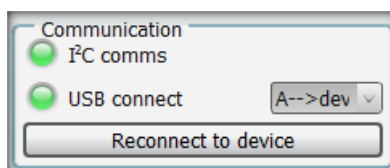
Figure 13: Communication Control
