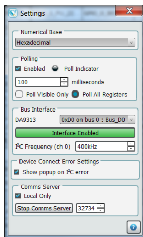
Figure 24: Settings
