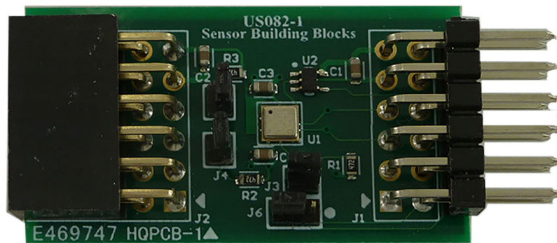
Figure 5. US082-ZMOD4510EVZ Evaluation Board (Top)
