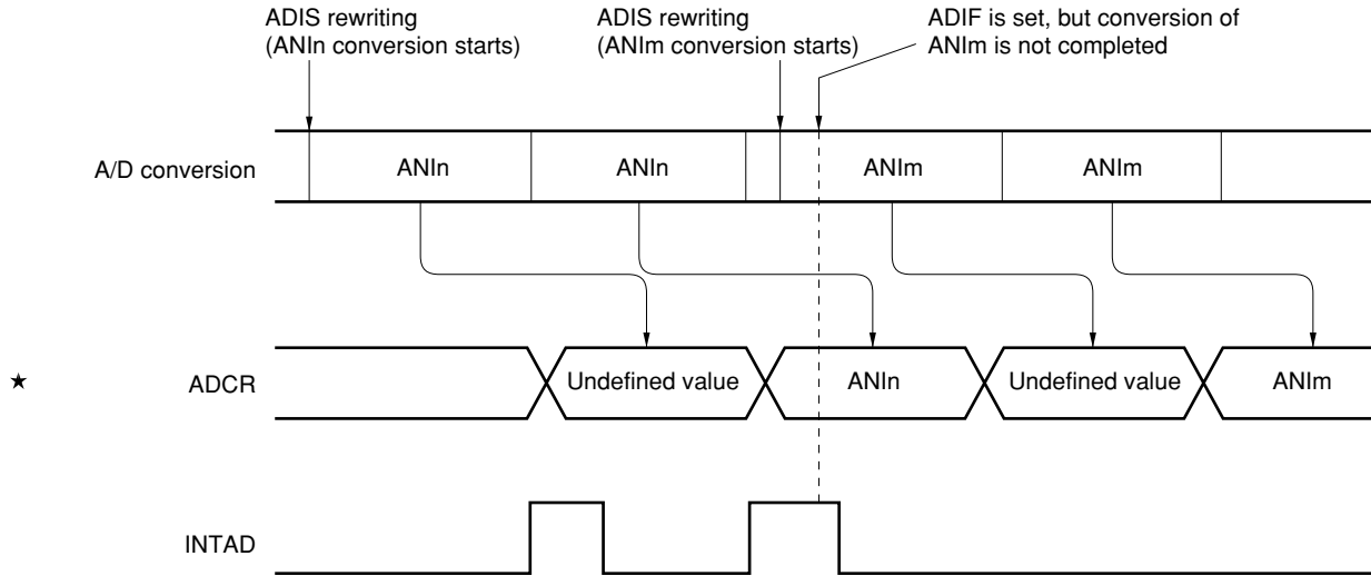
Figure 11-9. Timing of A/D Conversion End Interrupt Request Generation
