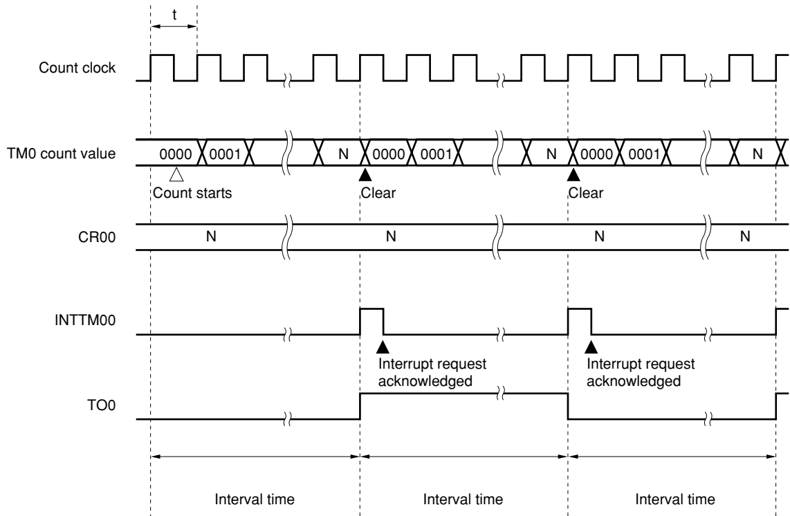
Figure 7-8. Timing of Interval Timer Operation
