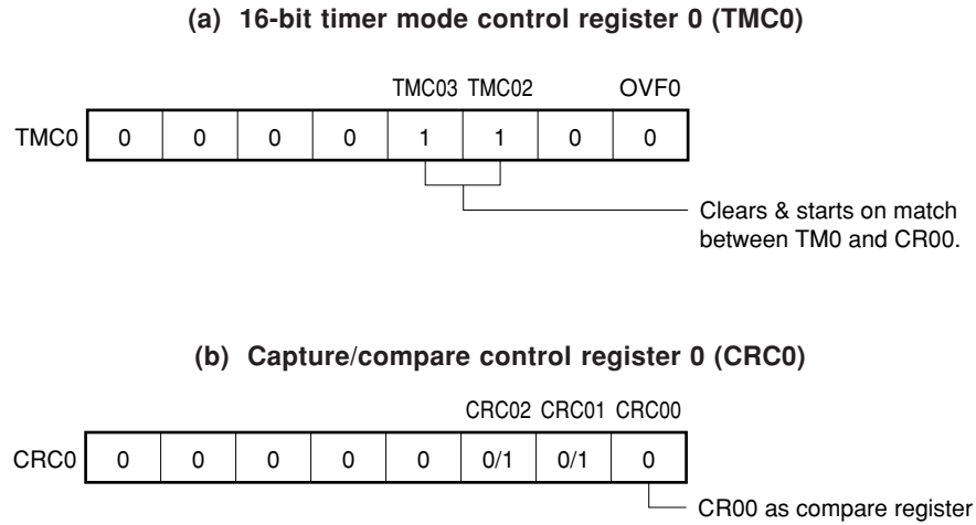
Figure 7-19. Control Register Settings in External Event Counter Mode
