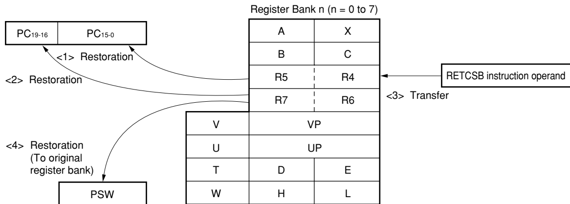
Figure 16-9. Return from BRKCS Instruction Software Interrupt (RETCSB Instruction Operation)
