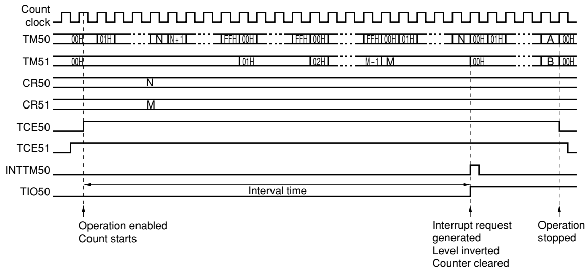
Figure 8-9. 16-Bit Resolution Cascade Mode
