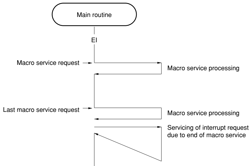
Figure 16-19. Operation at End of Macro Service When VCIE = 0
