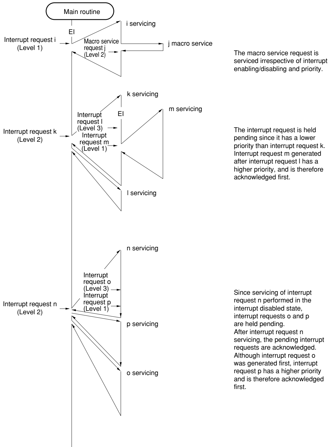
Figure 16-14. Examples of Servicing When Another Interrupt Request Is Generated During Interrupt Service (2/3)
