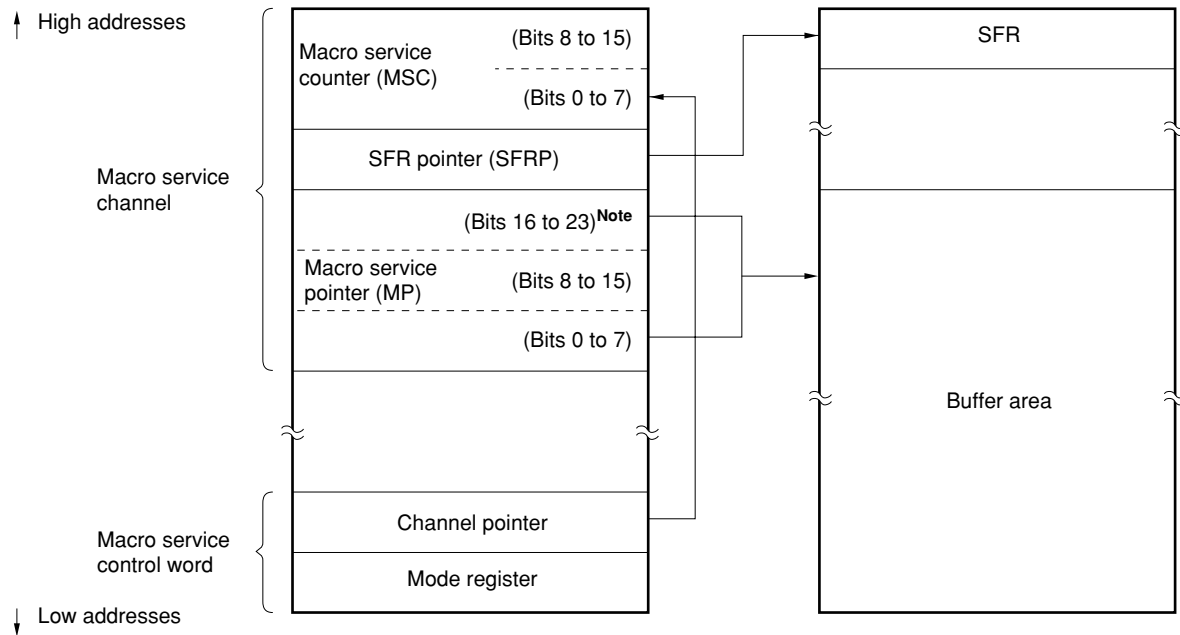
Figure 16-26. Type B Macro Service Channel
