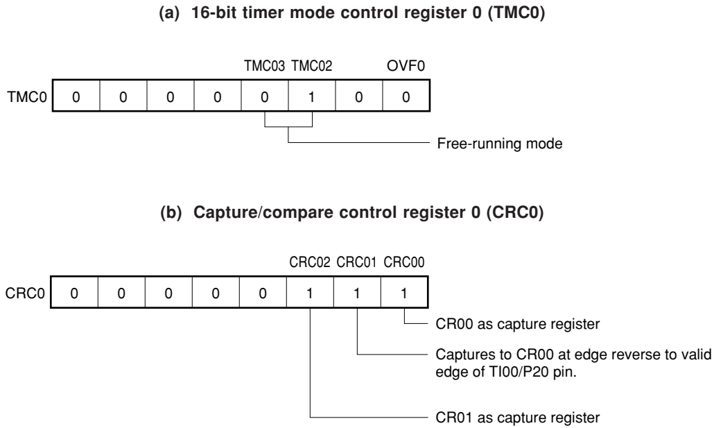
Figure 7-15. Control Register Settings for Pulse Width Measurement with Free-Running Counter and Two Capture Registers
