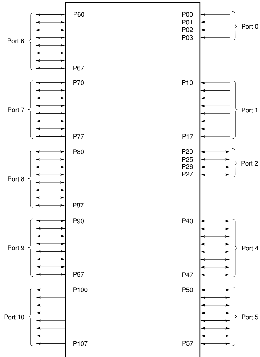
Figure 4-1. Port Types
