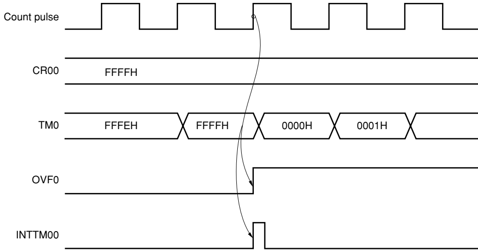
Figure 7-29. Operation Timing of OVFO Flag
