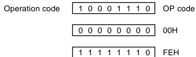
Figure 3-20: Direct addressing
