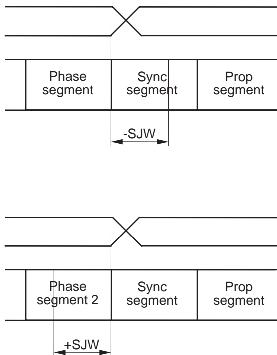
Figure 16-18: Bit Synchronization
