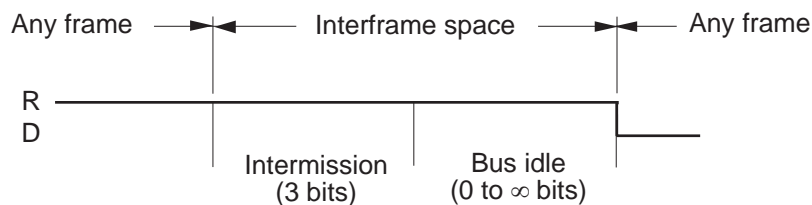
Figure 16-12: Interframe Space/Error Active
