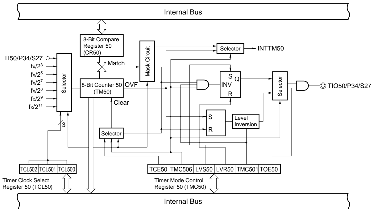
Figure 7-1: 8-Bit Timer/Event Counter 50 Block Diagram
