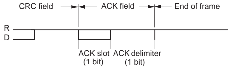
Figure 16-10: ACK Field
