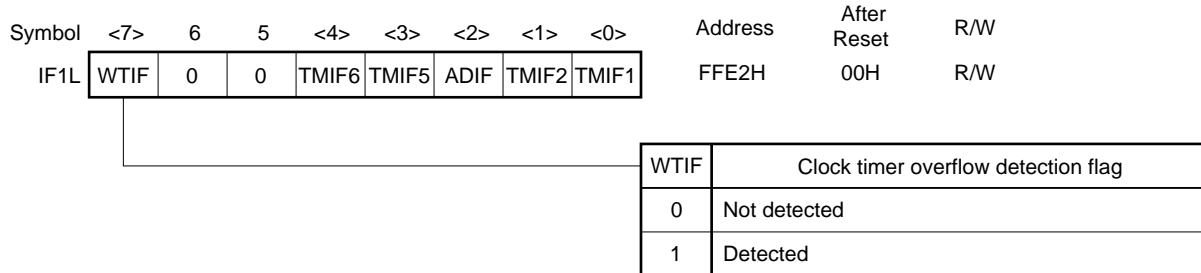
Figure 22-19. Interrupt Request Flag Register 1L Format
