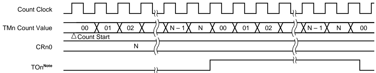
Figure 10-13. Square-wave Output Operation Timing
