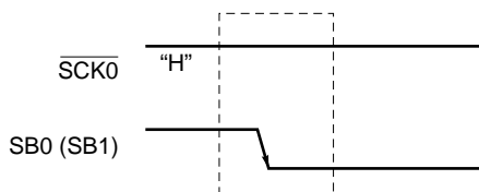
Figure 17-13. Command Signal
