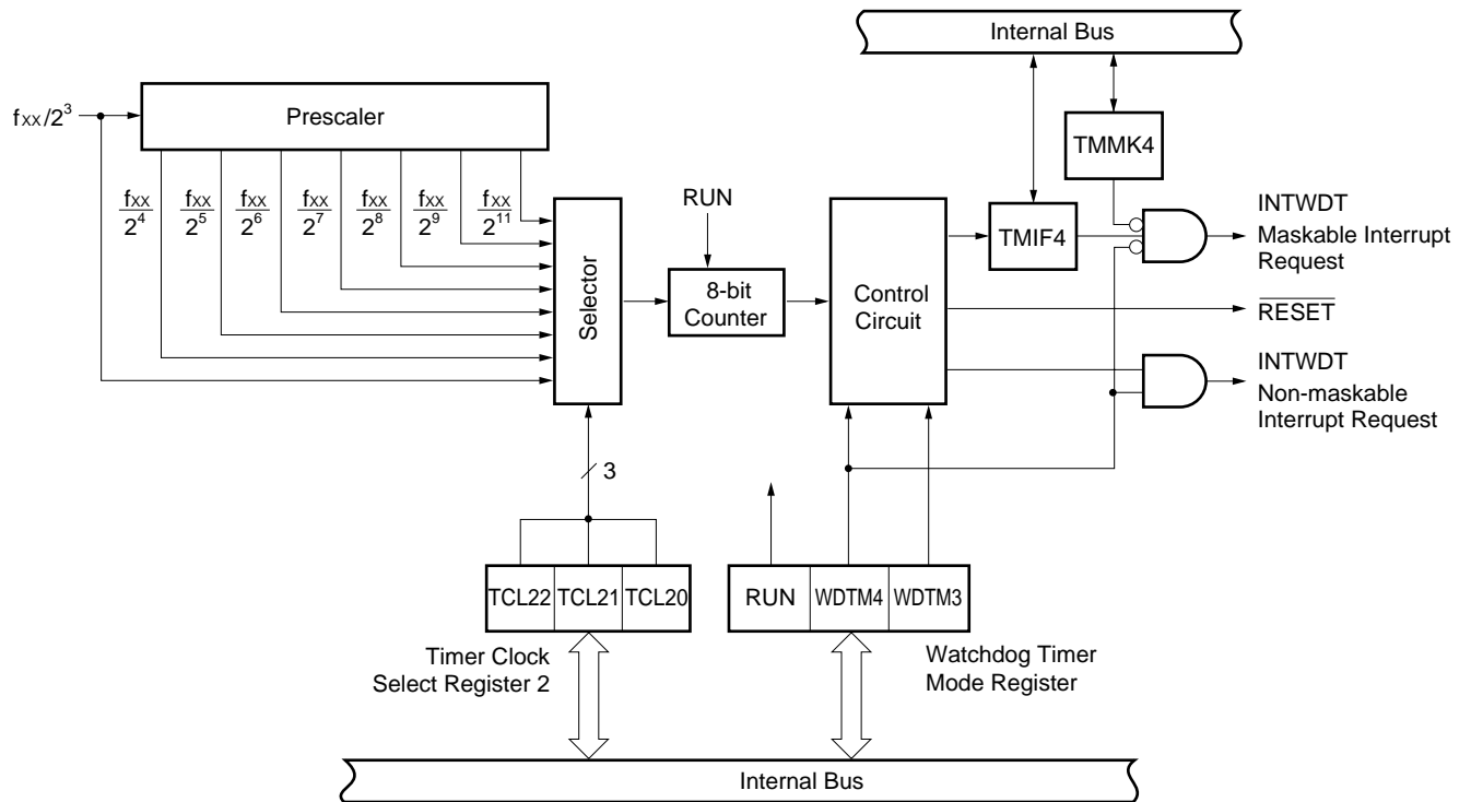
Figure 12-1. Watchdog Timer Block Diagram
