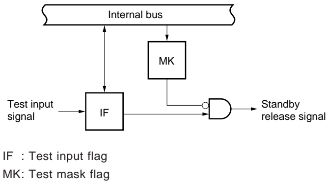
Figure 22-18. Basic Configuration of Test Function
