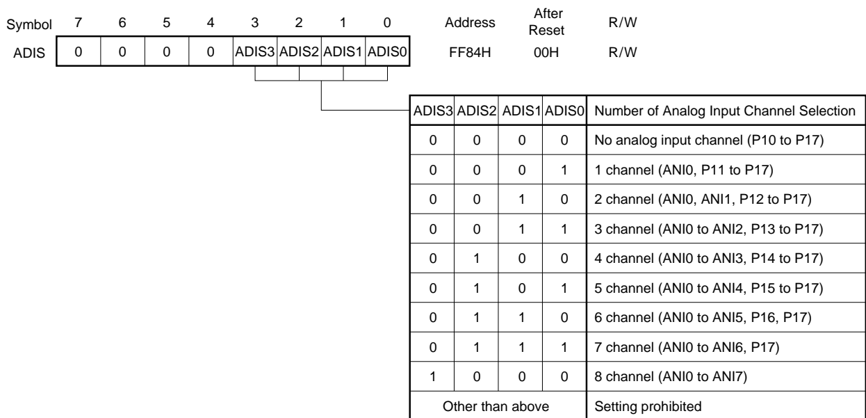
Figure 15-3. A/D Converter Input Select Register Format
