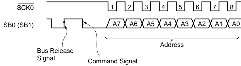
Figure 17-14. Addresses
