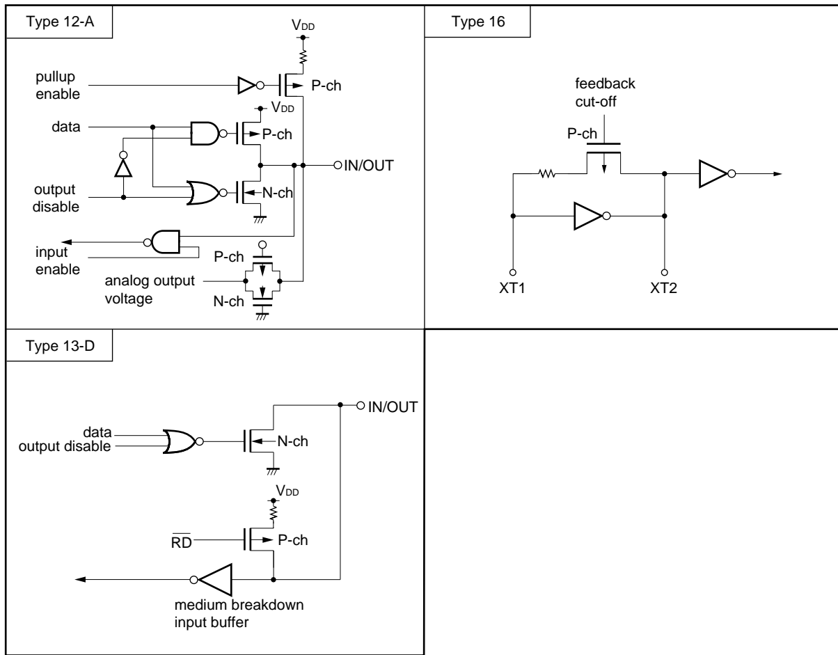
Figure 26-1. List of Pin Input/Output Circuits (2/2)
