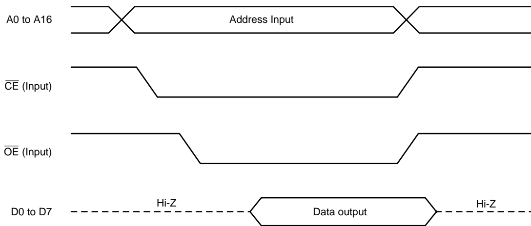
Figure 26-9. PROM Read Timing
