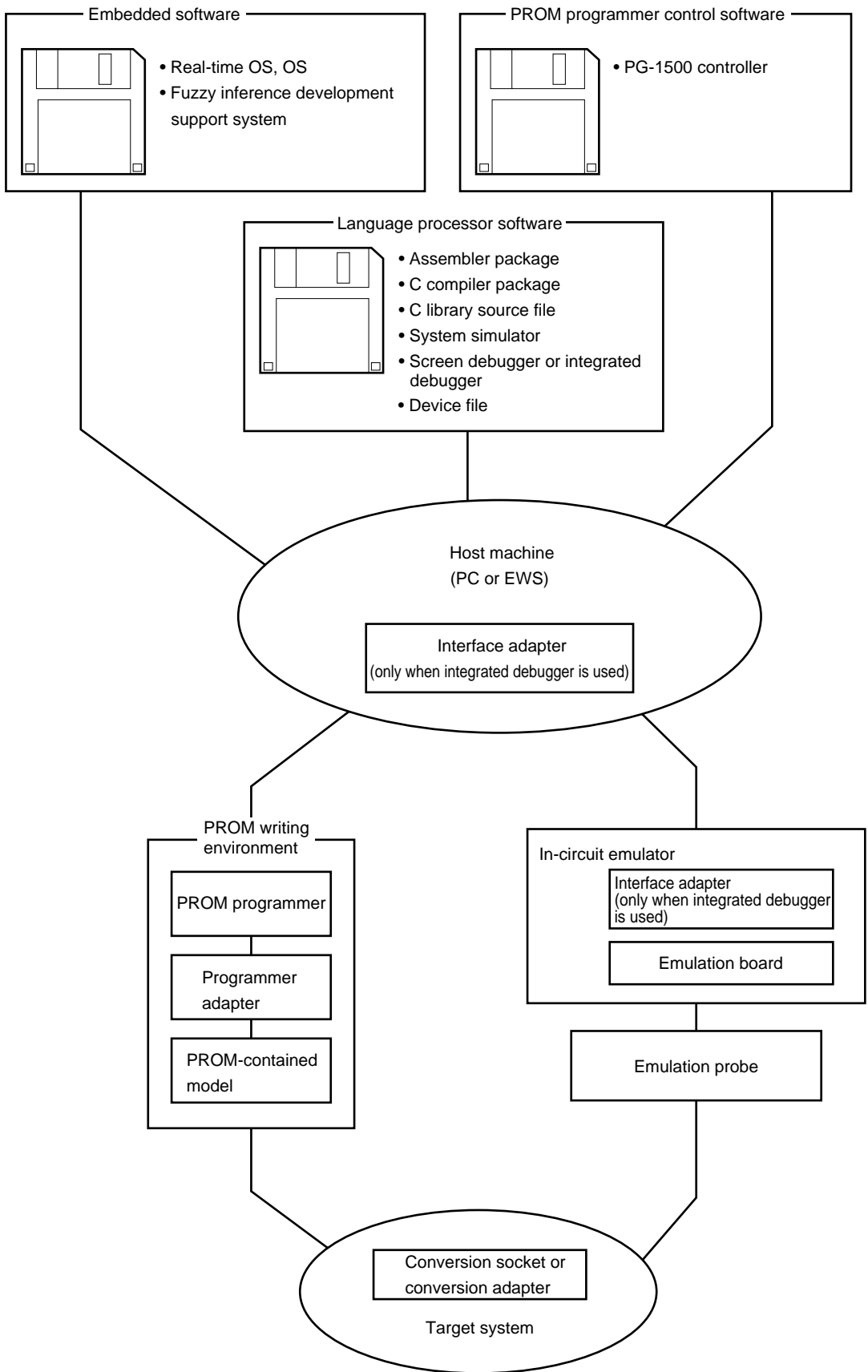
Figure B-1. Development Tool Configuration
