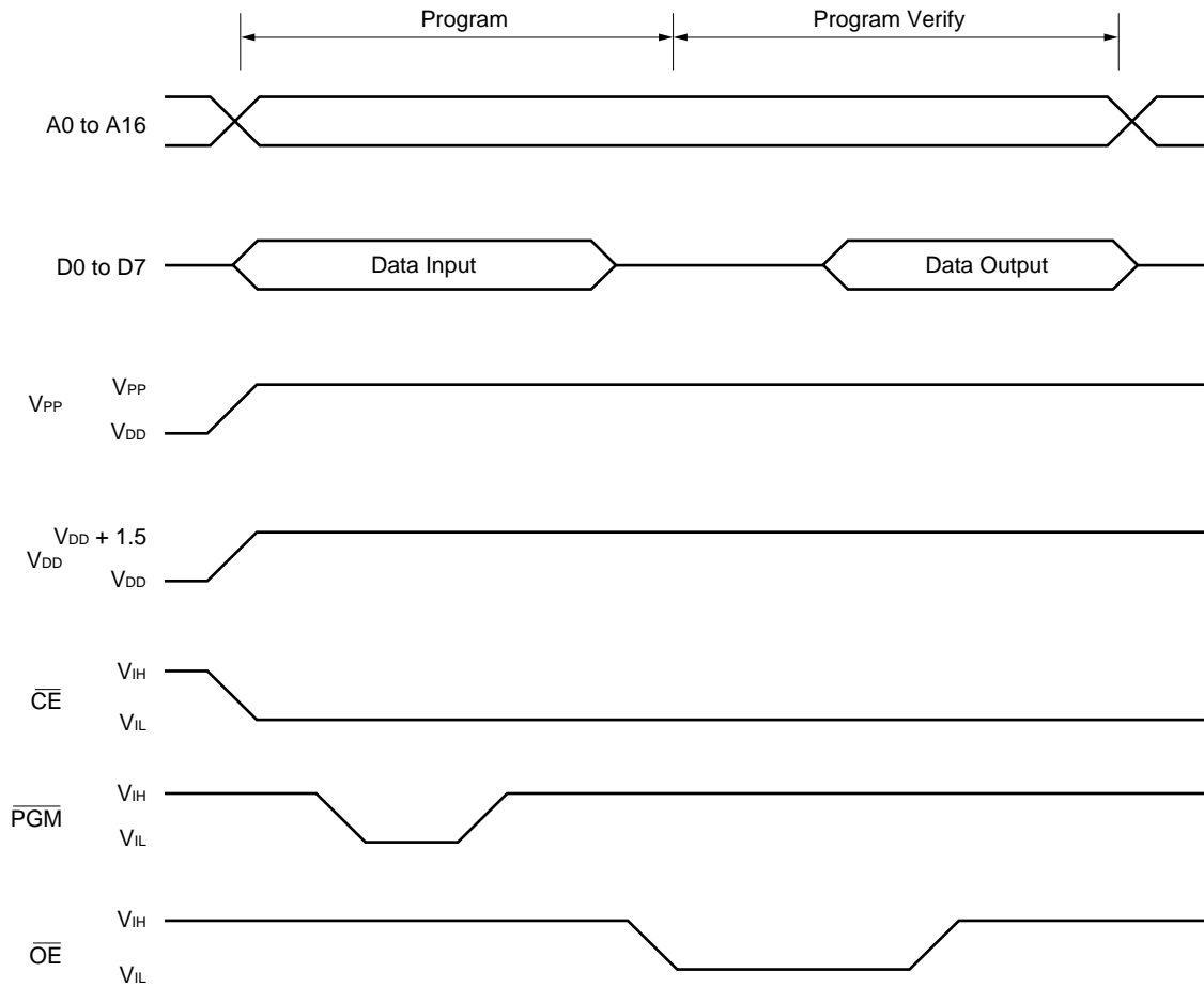
Figure 26-8. Byte Program Mode Timing
