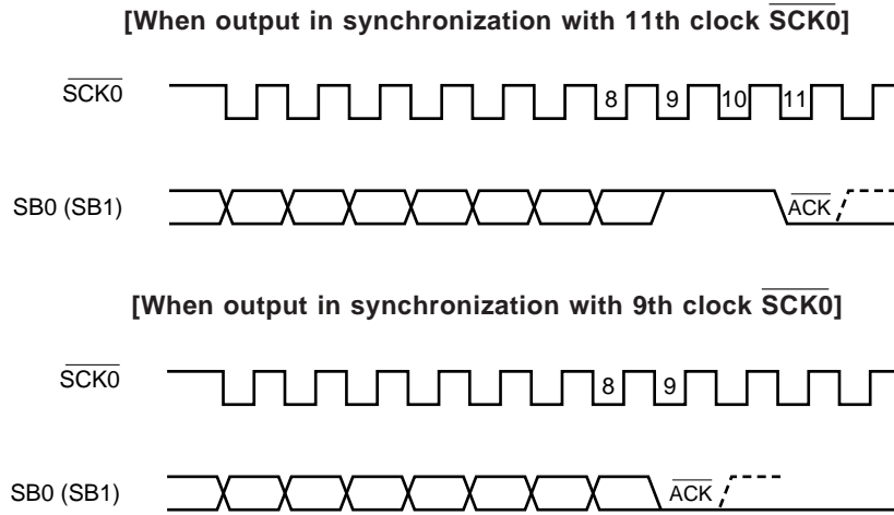
Figure 17-18. Acknowledge Signal
