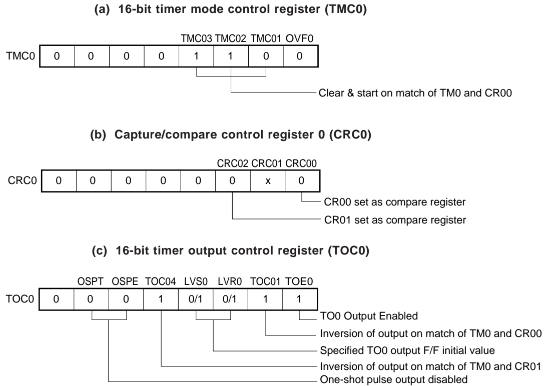
Figure 8-16. Control Register Settings for PPG Output Operation
