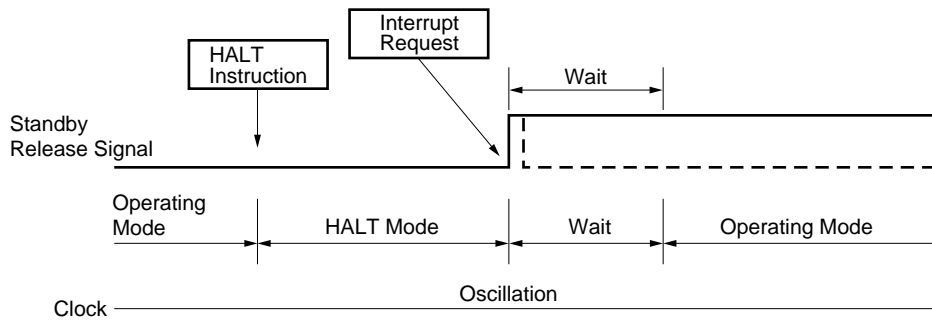
Figure 24-2. HALT Mode Release by Interrupt Request Generation
