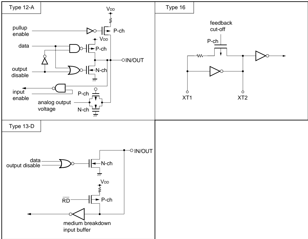
Figure 26-2. List of Pin Input/Output Circuits (2/2)
