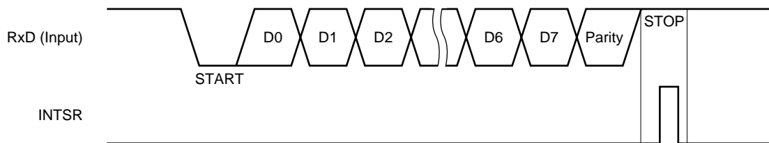
Figure 20-9. Asynchronous Serial Interface Reception Completion Interrupt Request Timing
