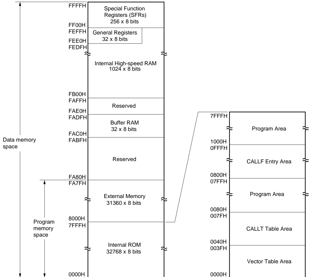
Figure 5-1. Memory Map ( \mu PD78074B, 78074BY)
