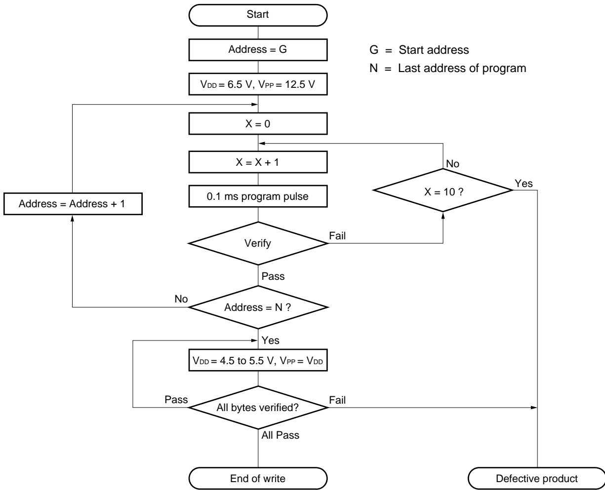
Figure 26-7. Byte Program Mode Flow Chart
