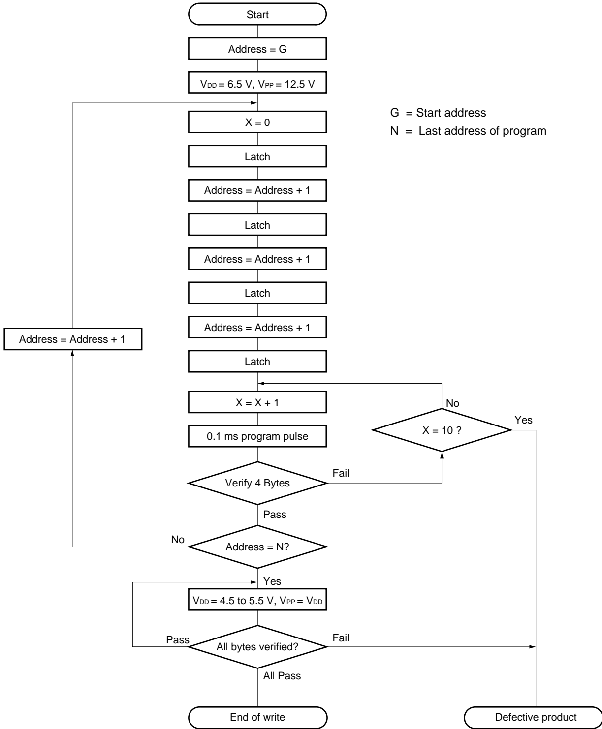
Figure 26-5. Page Program Mode Flowchart
