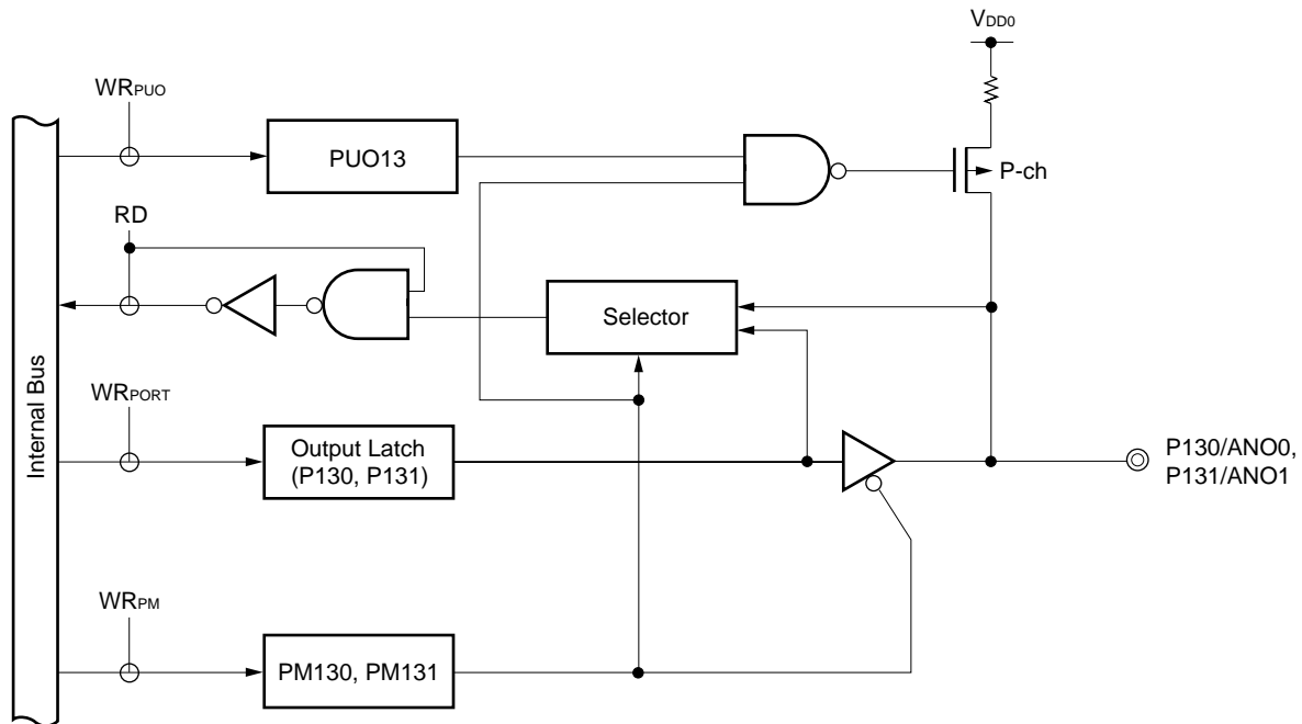
Figure 6-23. Block Diagram of P130 and P131
