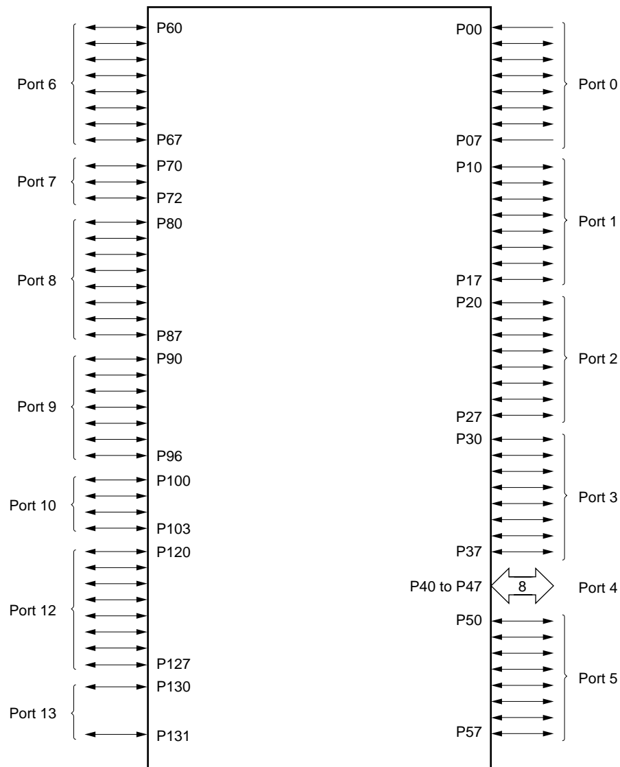
Figure 6-1. Port Types
