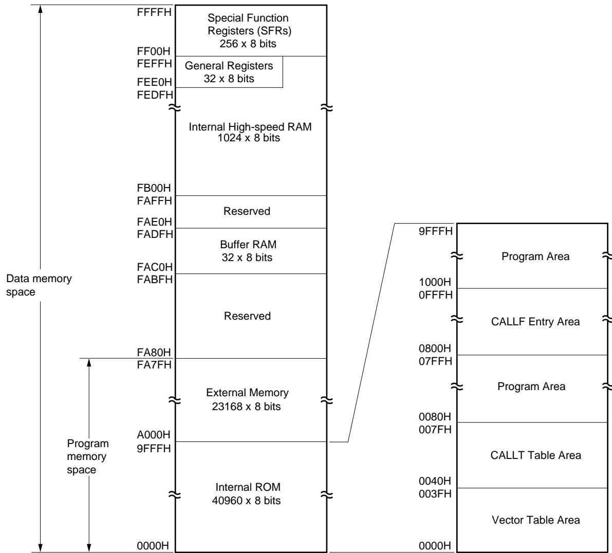
Figure 5-2. Memory Map ( \mu PD78075B, 78075BY)
