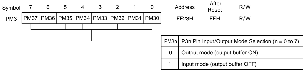
Figure 14-3. Port Mode Register 3 Format
