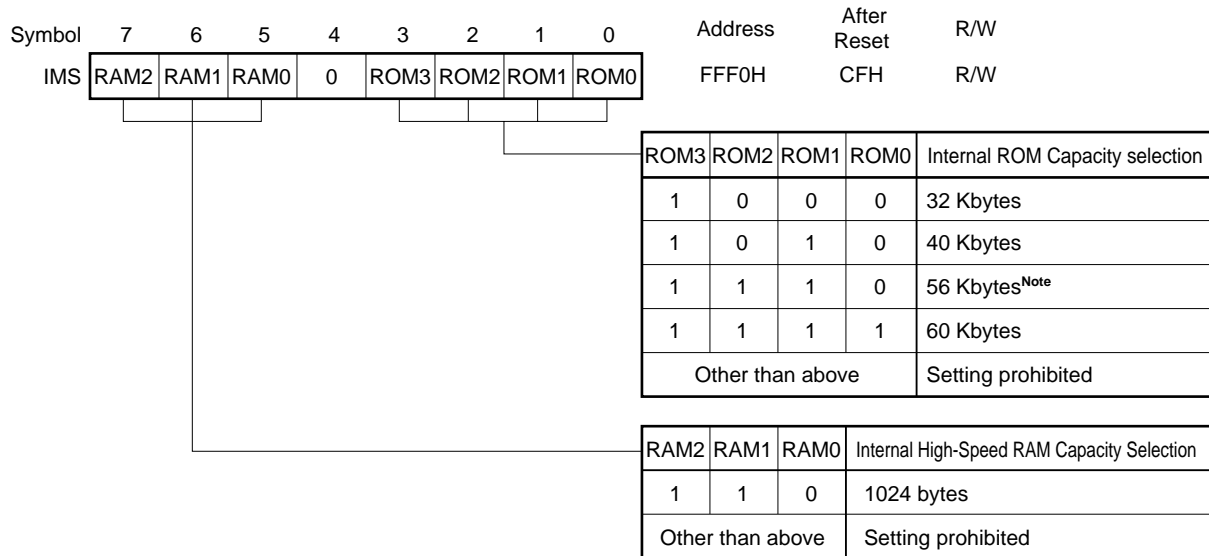
Figure 26-3. Internal Memory Size Switching Register Format
