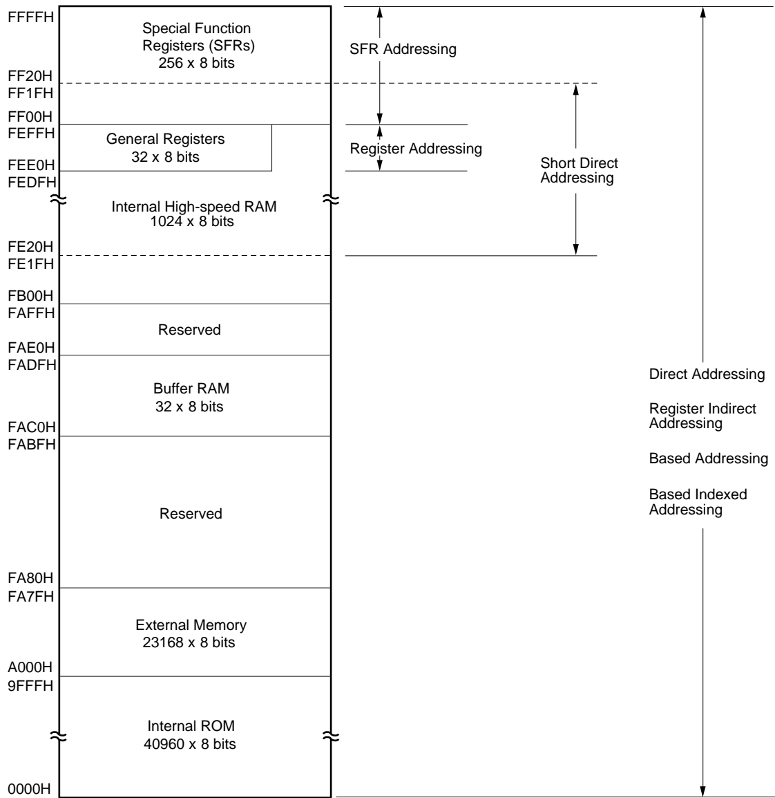
Figure 5-4. Data Memory Addressing ( \mu PD78075B, 78075BY)
