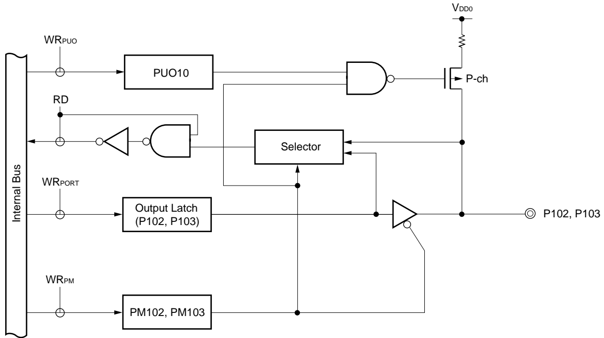
Figure 6-21. Block Diagram of P102 and P103
