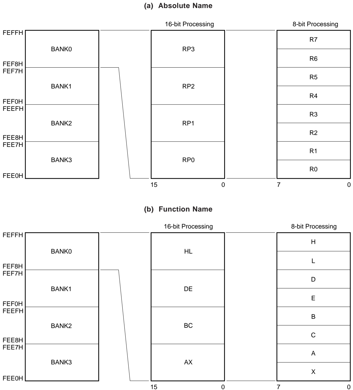
Figure 5-10. General Register Configuration
