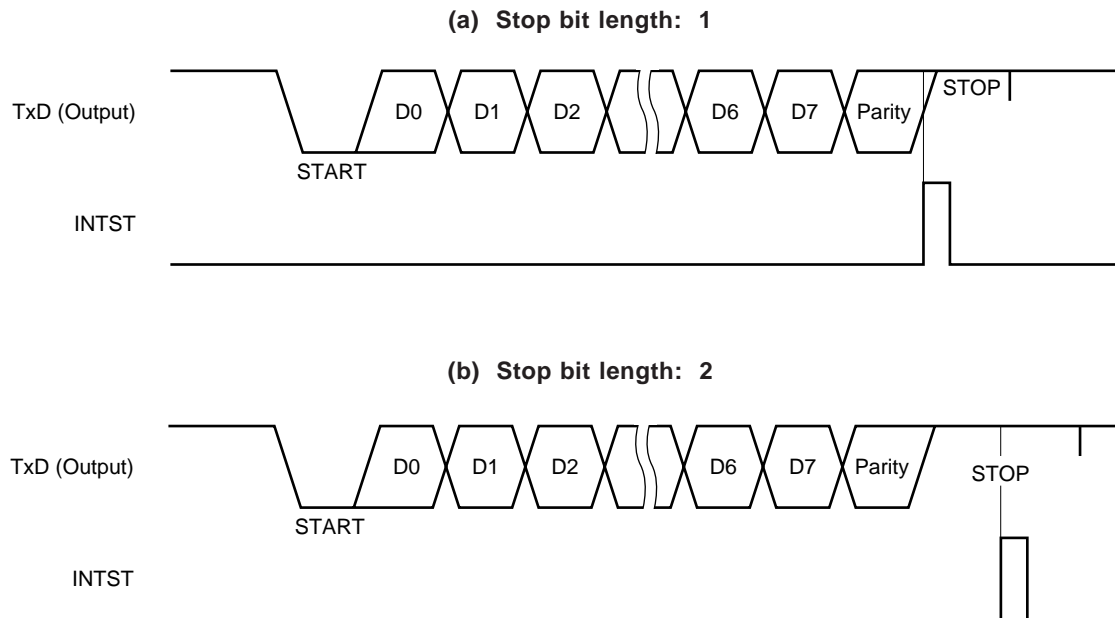
Figure 20-8. Asynchronous Serial Interface Transmission Completion Interrupt Request Timing
