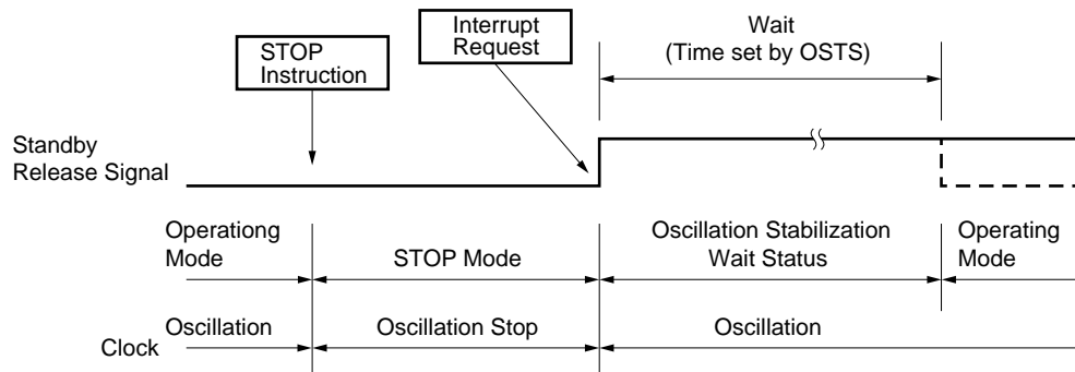
Figure 24-4. STOP Mode Release by Interrupt Request Generation
