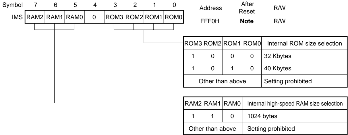
Figure 23-3. Internal Memory Size Switching Register Format
