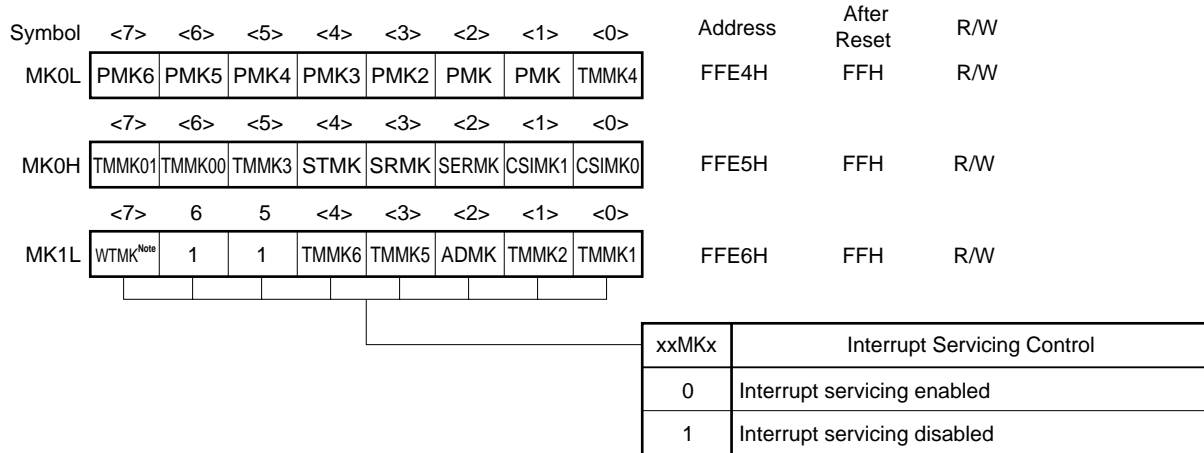
Figure 22-3. Interrupt Mask Flag Register Format
