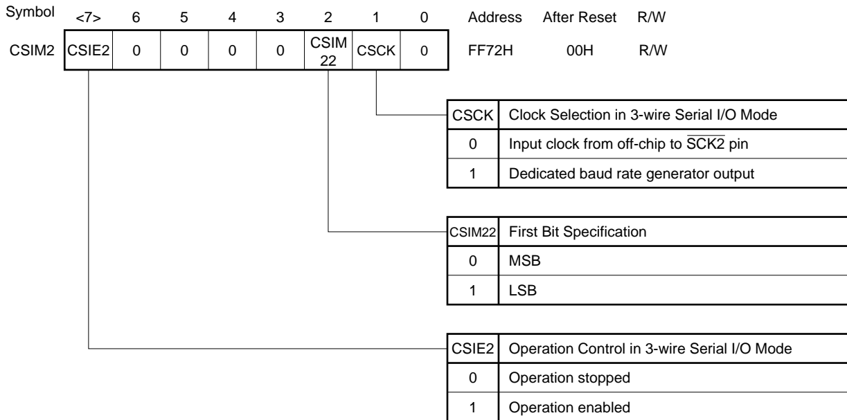
Figure 20-3. Serial Operating Mode Register 2 Format
