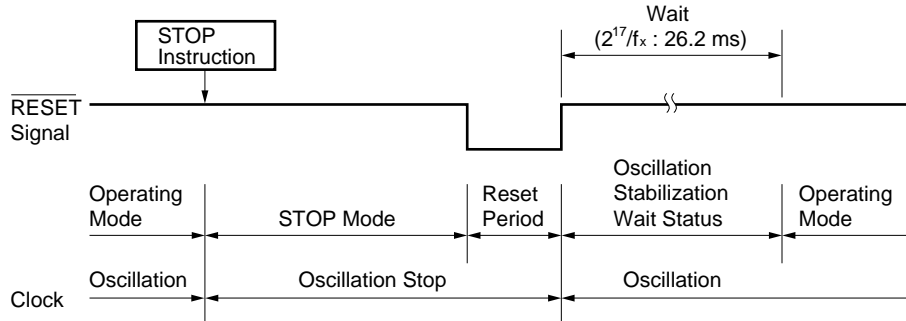
Figure 24-5. Release by STOP Mode \overline{\text{RESET}} Input
