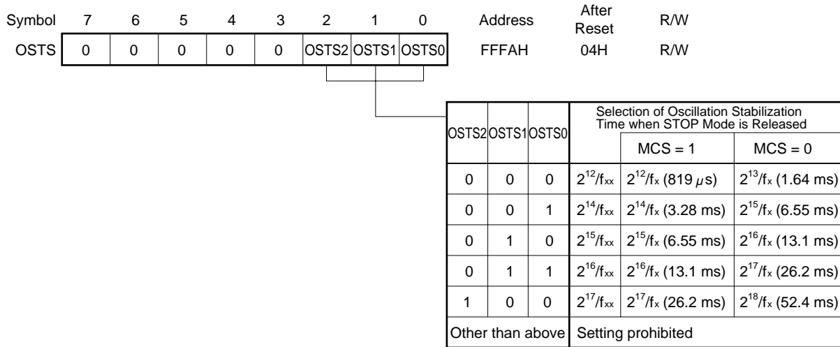
Figure 24-1. Oscillation Stabilization Time Select Register Format
