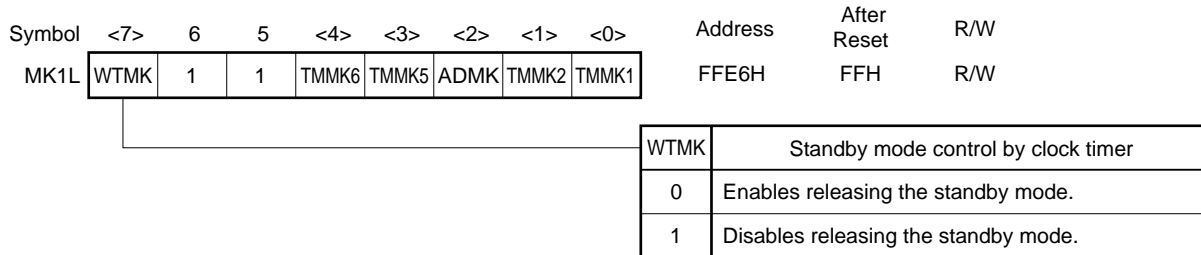
Figure 22-20. Interrupt Mask Flag Register 1L Format
