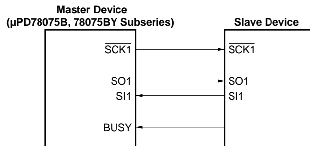
Figure 19-18. System Configuration when the Busy Control Option is Used
