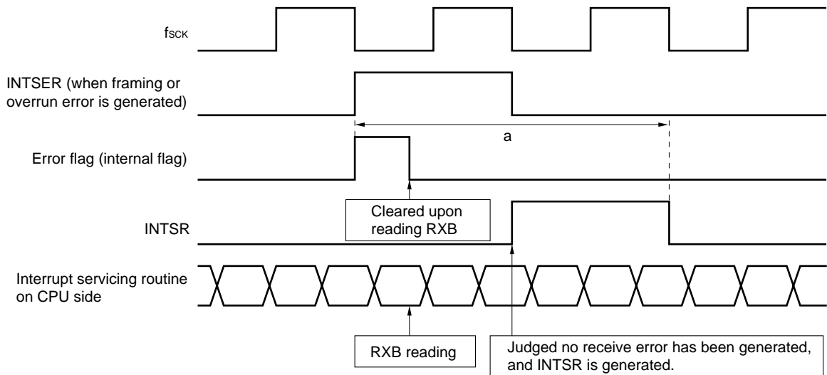
Figure 20-14. Receive Completion Interrupt Generation Timing (when ISRM = 1)
