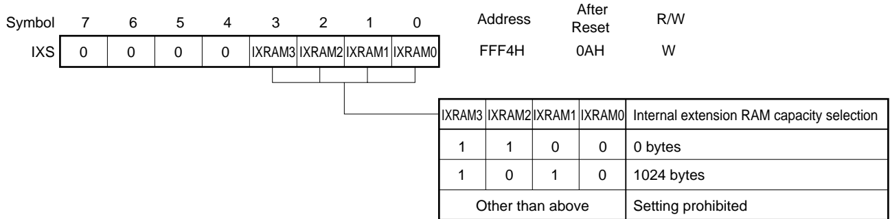
Figure 26-4. Internal Extension RAM Size Switching Register Format
