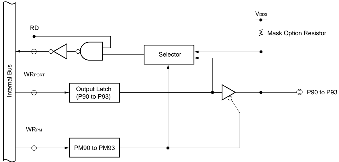
Figure 6-18. Block Diagram of P90 to P93
