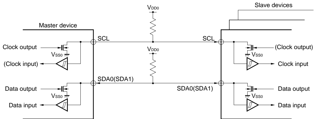
Figure 18-21. Pin Configuration
