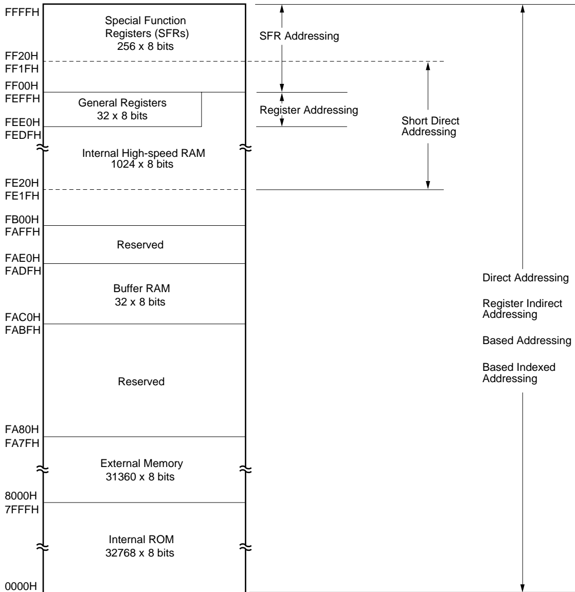
Figure 5-3. Data Memory Addressing ( \mu PD78074B, 78074BY)
