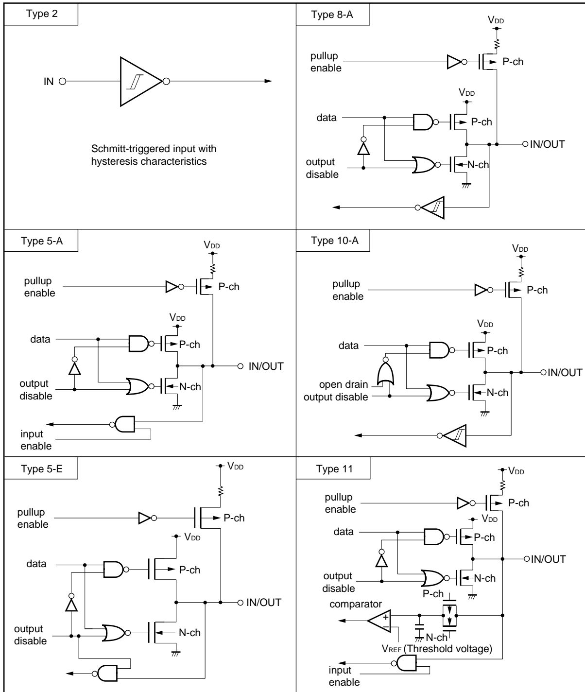
Figure 26-2. List of Pin Input/Output Circuits (1/2)
