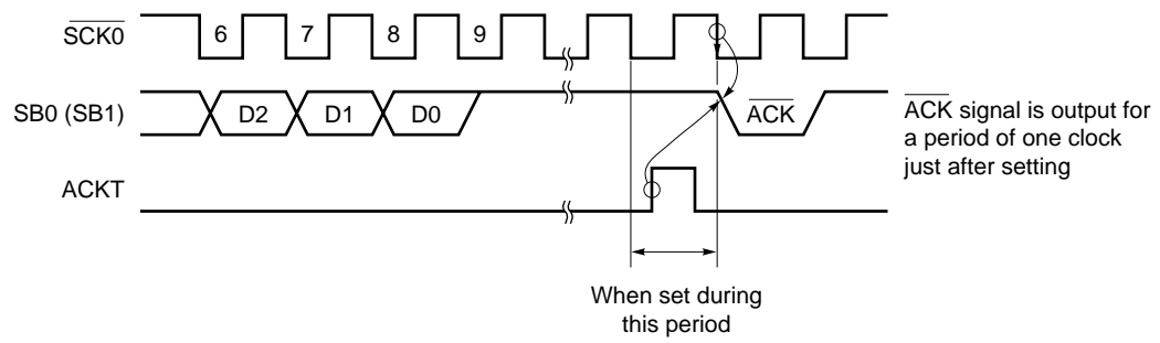
Figure 17-22. ACKT Operation
