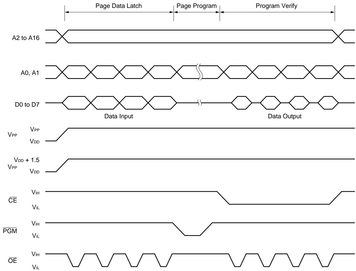
Figure 26-6. Page Program Mode Timing
