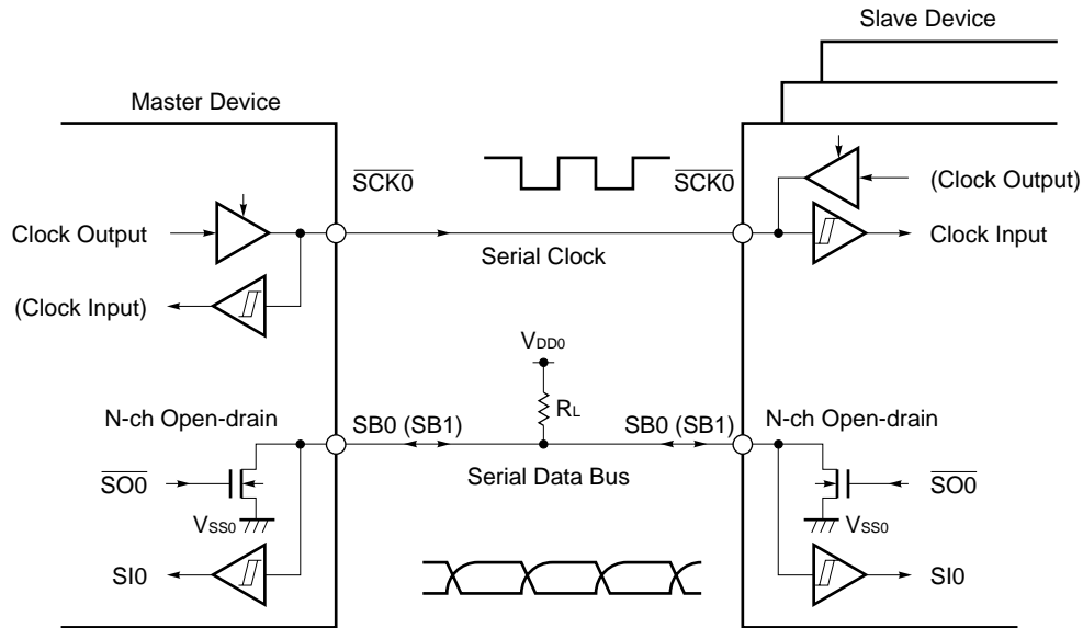
Figure 17-26. Pin Configuration
