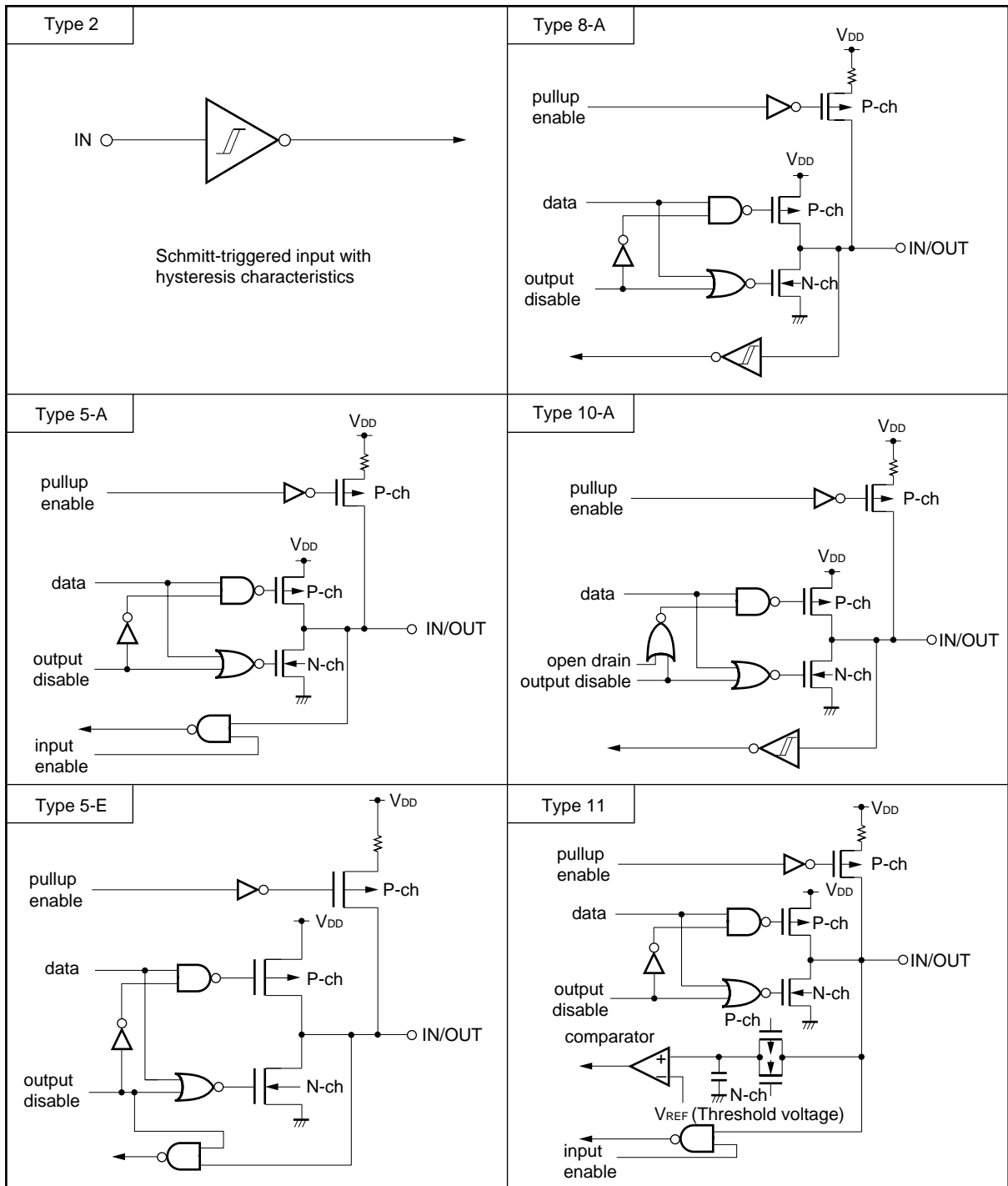
Figure 26-1. List of Pin Input/Output Circuits (1/2)
