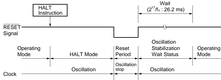
Figure 24-3. HALT Mode Release by \overline{\text{RESET}} Input
