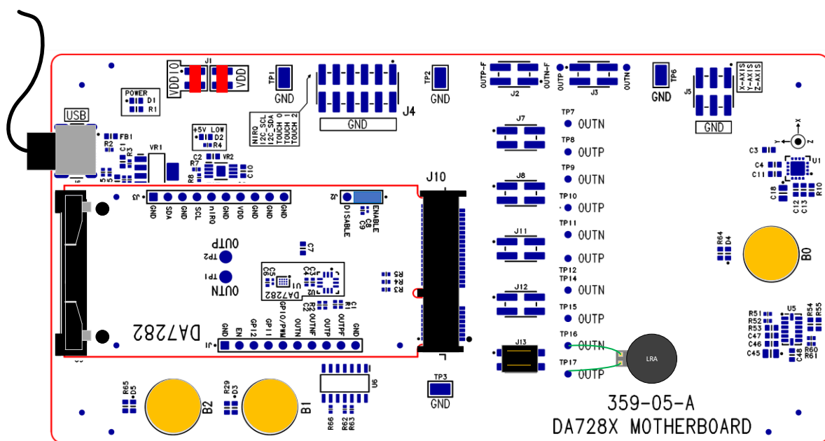
Figure 3: Motherboard Operation
