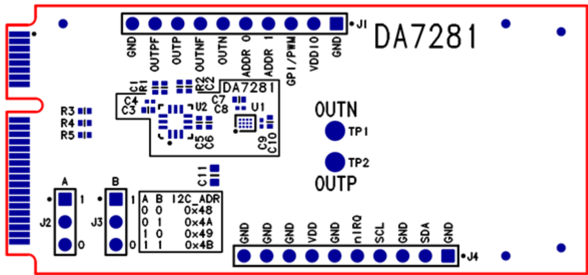
Figure 1: 359-07-X PCB
