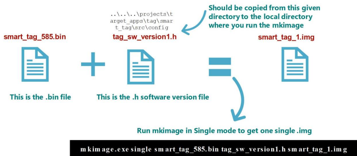
Figure 30: Create a Single Image from a Binary
