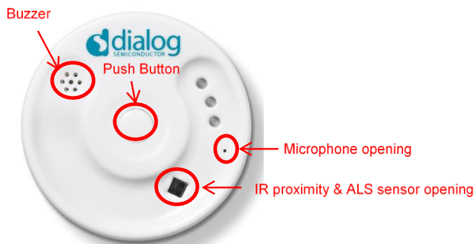
Figure 32: DA14585 IoT MSK Enclosure: Top View
