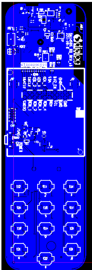
Figure 24: DA14585 Voice RCU Reference Design Rev. B - Top View
