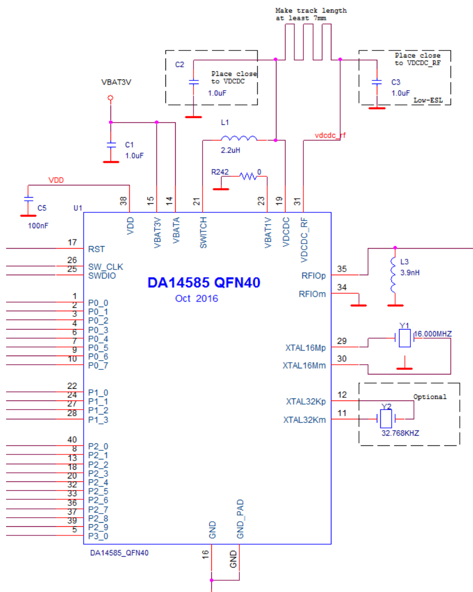
Figure 8: DA14585 System Schematic
