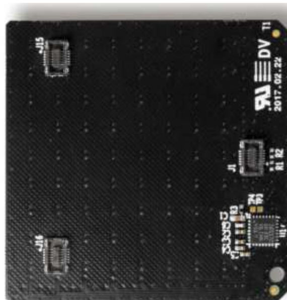
Figure 5: Trackpad Daughterboard (Rev B) – Bottom View
