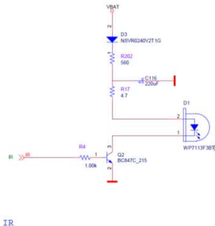
Figure 14: IR LED Schematic
