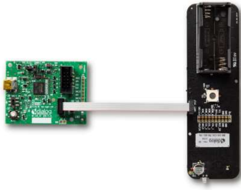
Figure 40: Connection of the DA14585 Voice RCU PCB to the CIB Programming Board
