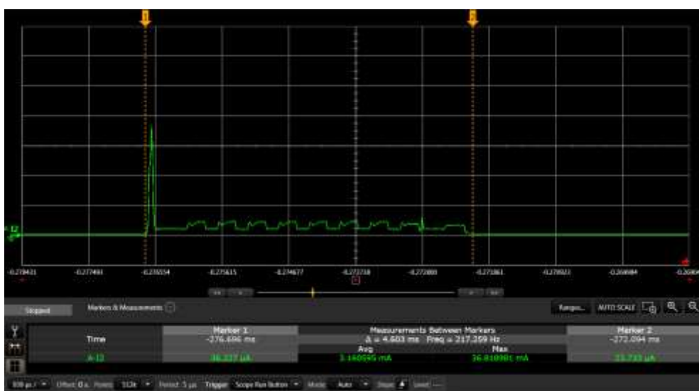
Figure 30: DA14585 Voice RCU Reference Design – Current during Touch Pad Scan Pulse
