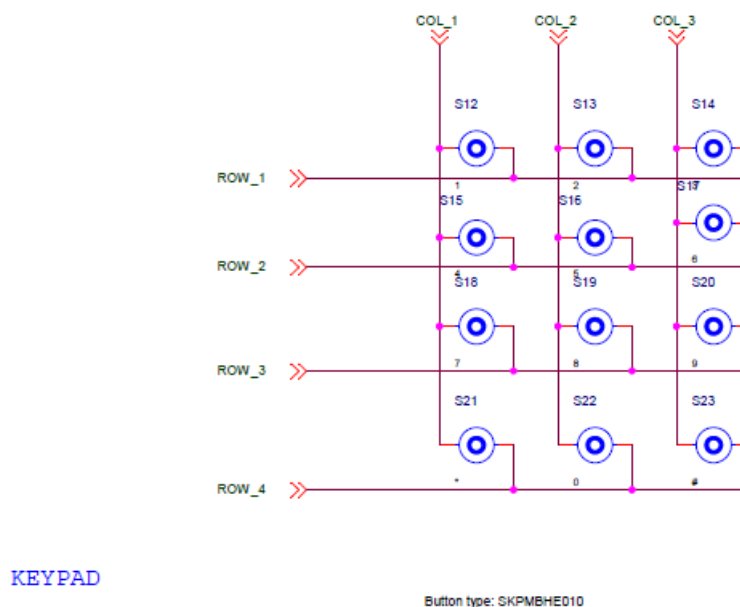
Figure 19: Keypad Matrix Schematic
