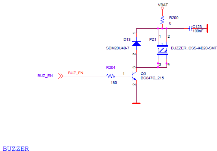
Figure 15: Buzzer Schematic
