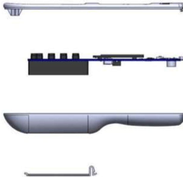
Figure 36 : DA14585 Voice RCU Reference Design Enclosure - Side Exploded View
