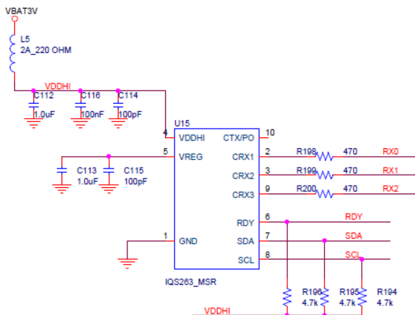
Figure 11: Capacitive Touch Controller Schematic (Trackpad)
