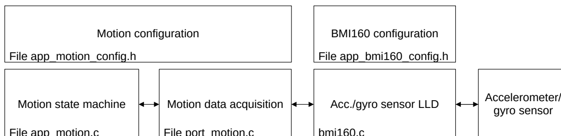
Figure 8: Motion Module Block Diagram
