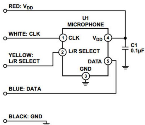
Figure 23: Microphone Pins and Cables
