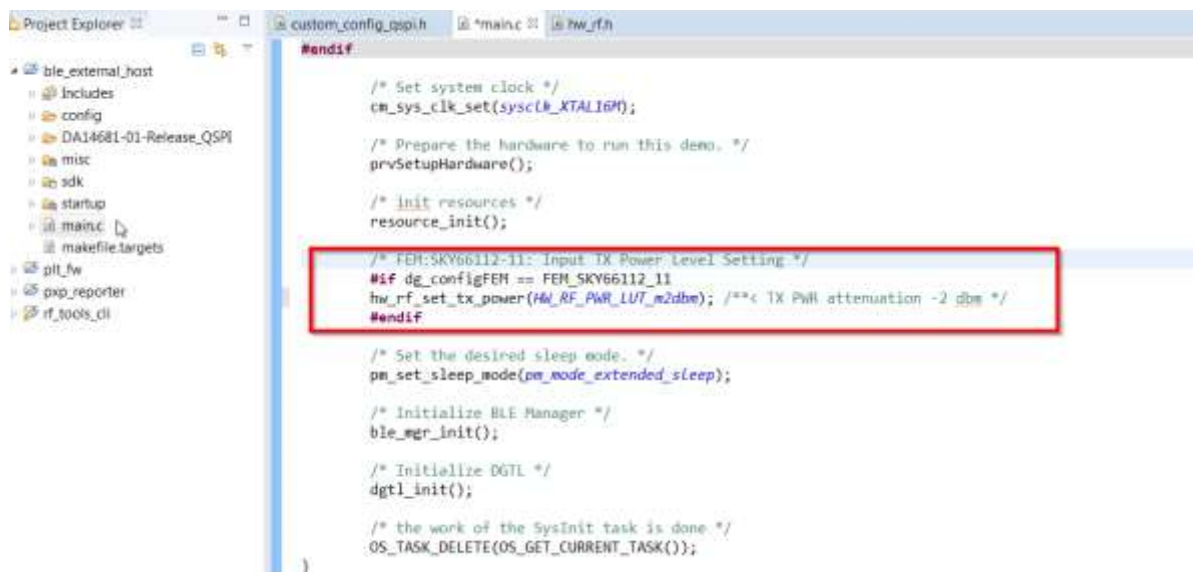
Figure 21: Configure DA14681 Power Output Level at -2 dBm
