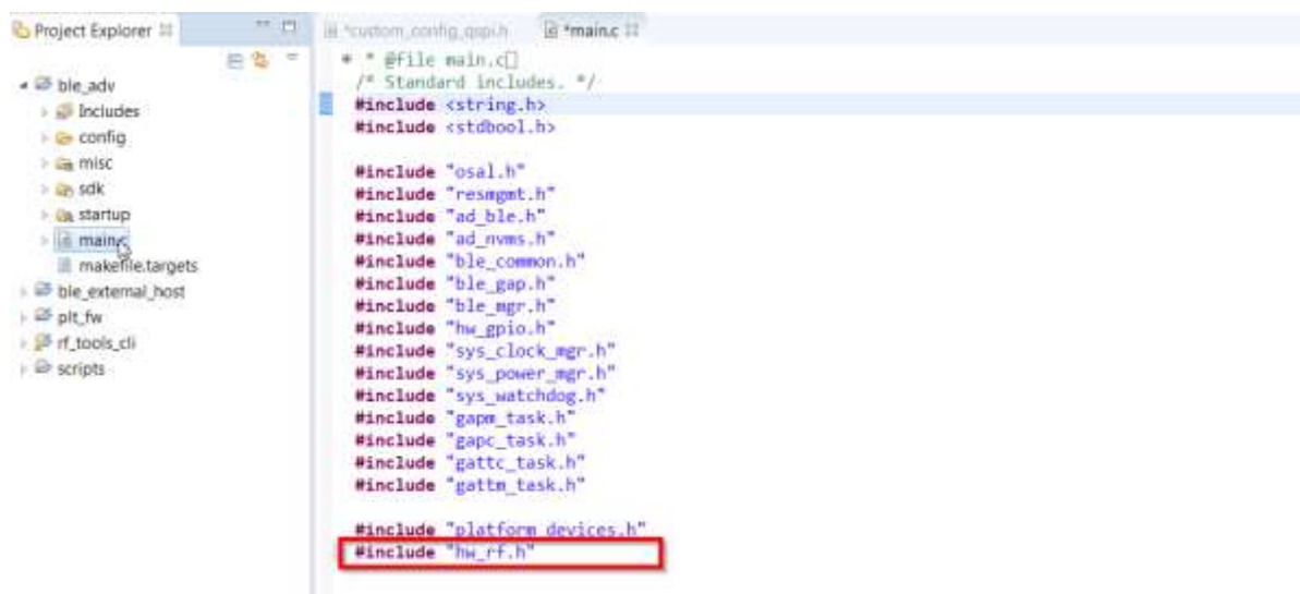
Figure 46: Include hw_rf.h in main.c
