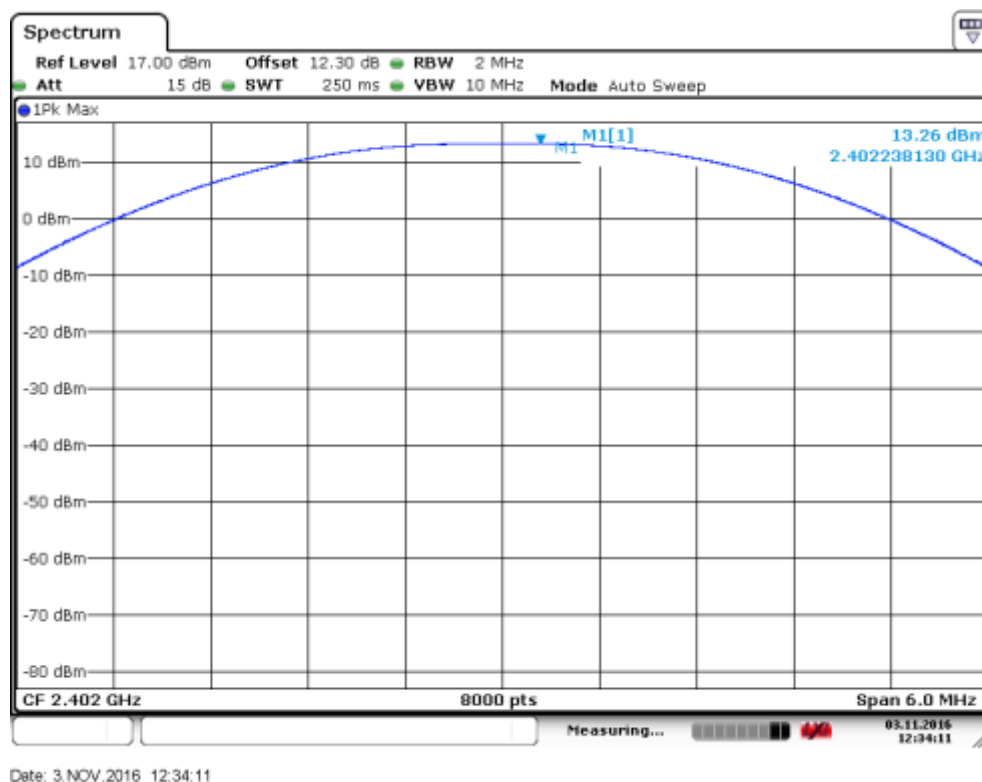
Figure 32: Maximum Output Power, CH00, VCC2 = 1.2 V
