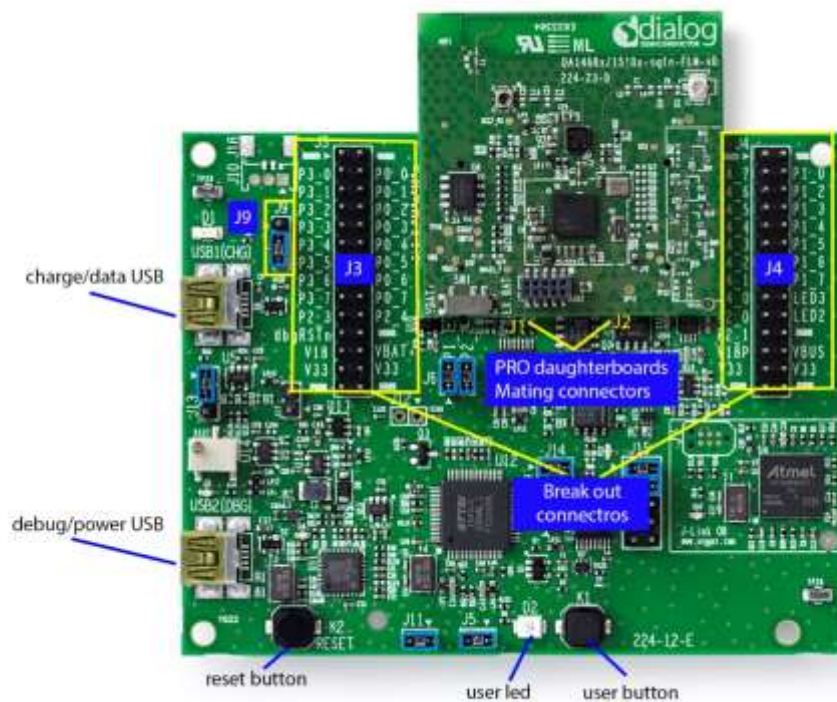
Figure 3: Range Extender (224-23-D) on a DA1468x Dev.Kit PRO Motherboard
