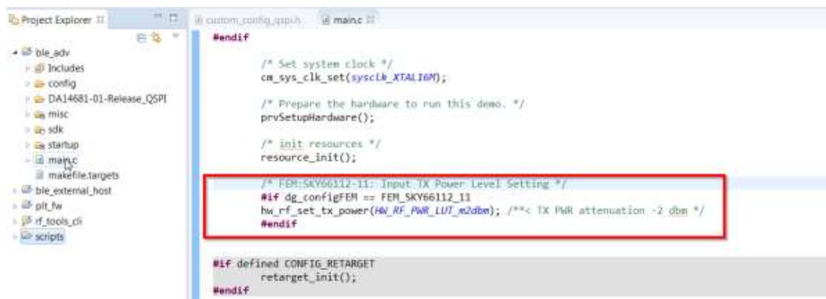
Figure 45: Configure DA14681 Power Output Level at -2 dBm
