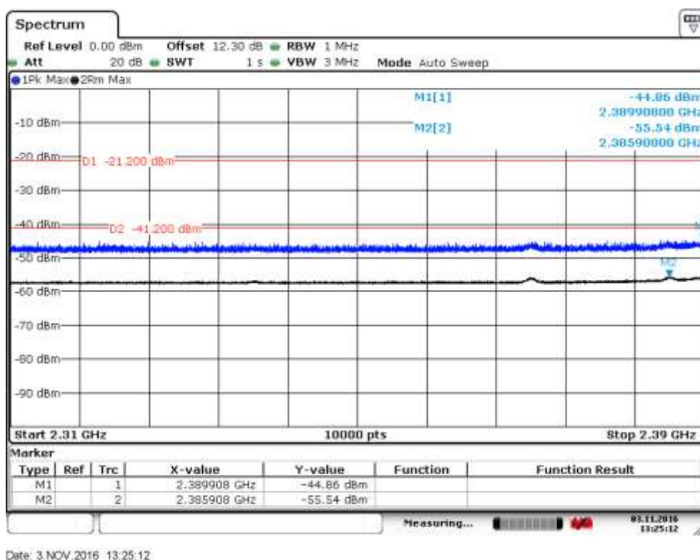
Figure 41: Emissions in Restricted Band RA 2.31 GHz to 2.39 GHz, CH00
