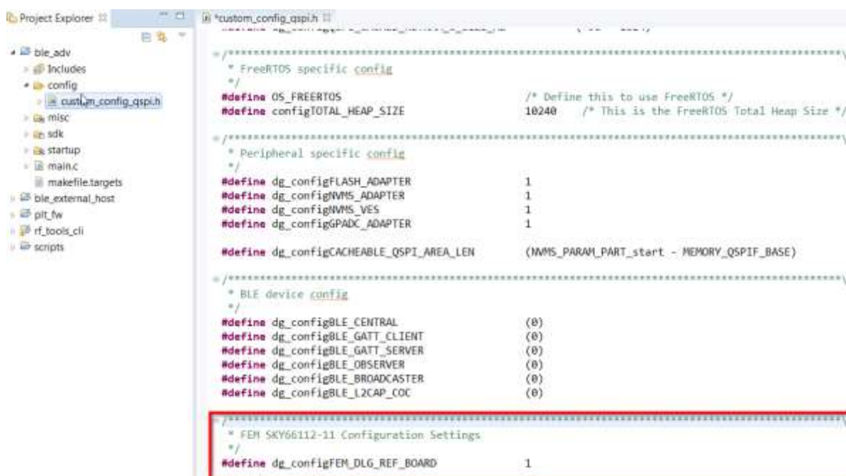
Figure 43: Enable FEM Driver in custom_config_qspi.h
