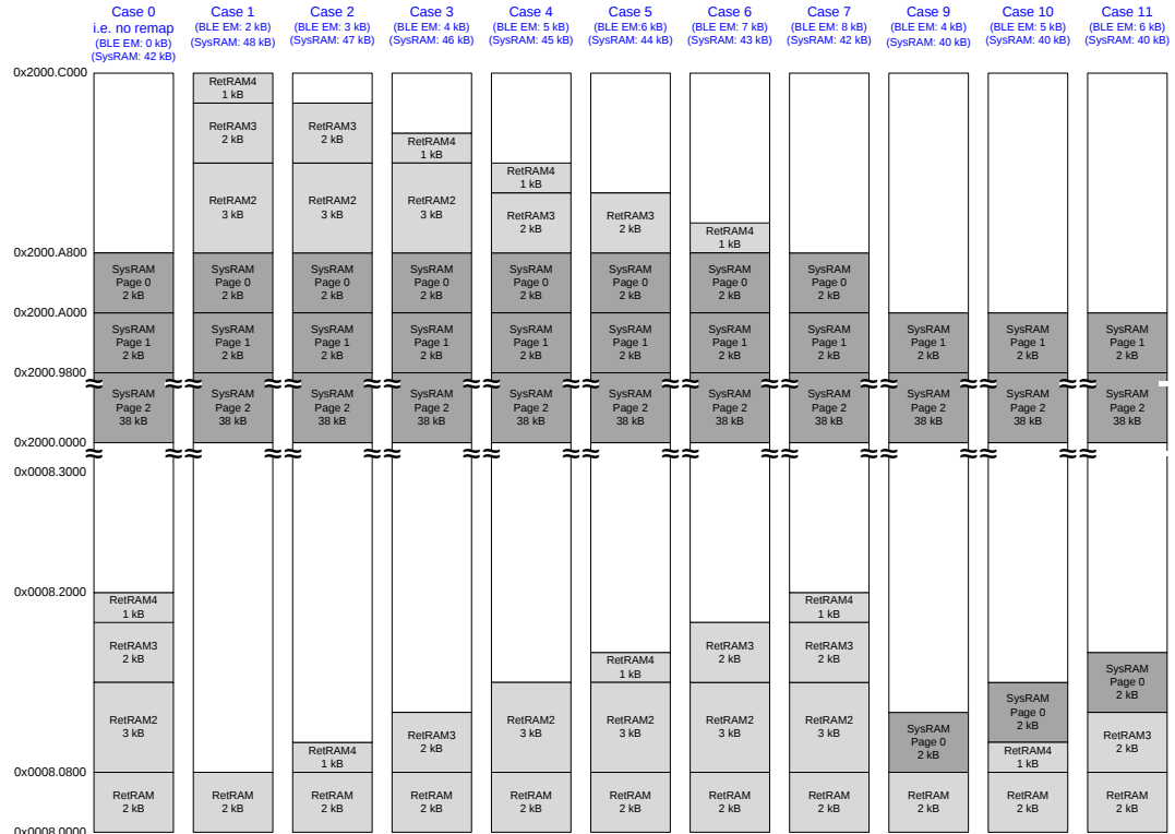
Figure 24: Memory Configurations (0..11)
