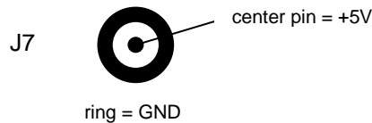
Figure 3-4: Power supply connector J7 (board front view)
