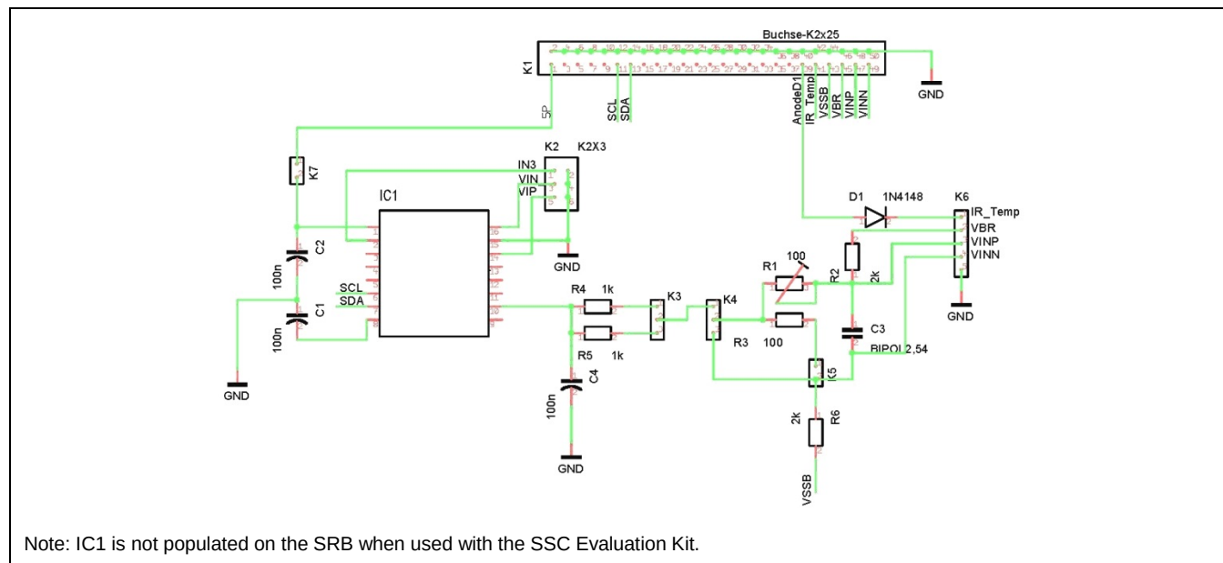
Figure 2.2 SSC Sensor Replacement Board (SRB) Schematic
