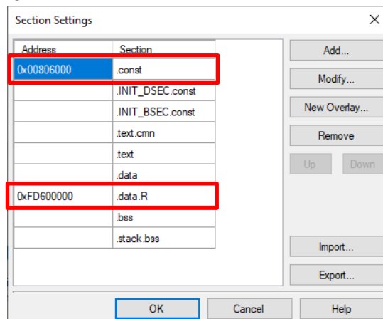
Figure 4-22. Setting in the subproject PE3
