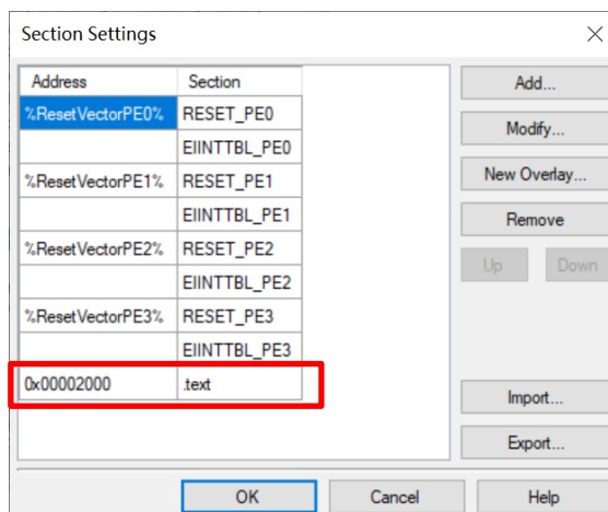
Figure 4-18. Setting in the main project u2a16_startup
