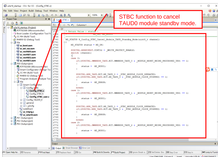
Figure 5-7. Cancel stand-by mode function for TAUD
