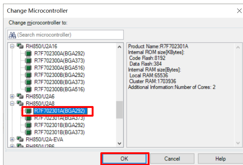
Figure 4-11. Select device to be changed
