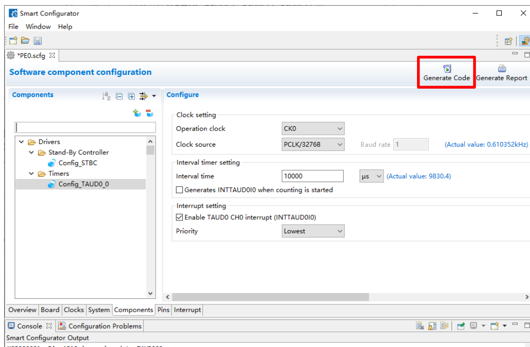
Figure 5-8. Generating code
