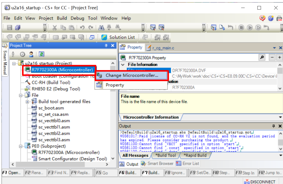
Figure 4-9. Change Microcontroller
