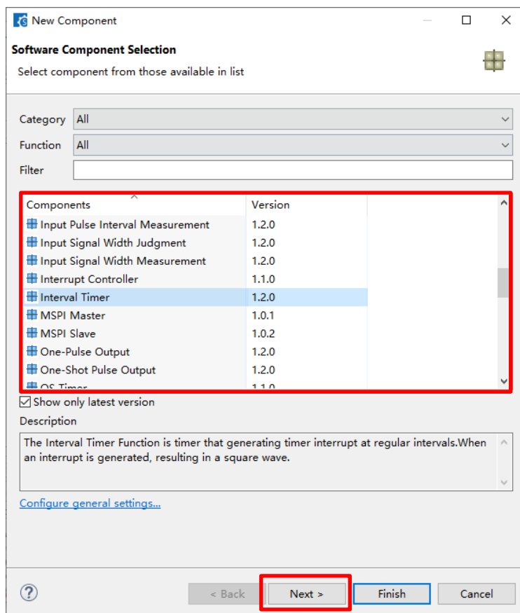
Figure 5-3. Select components
