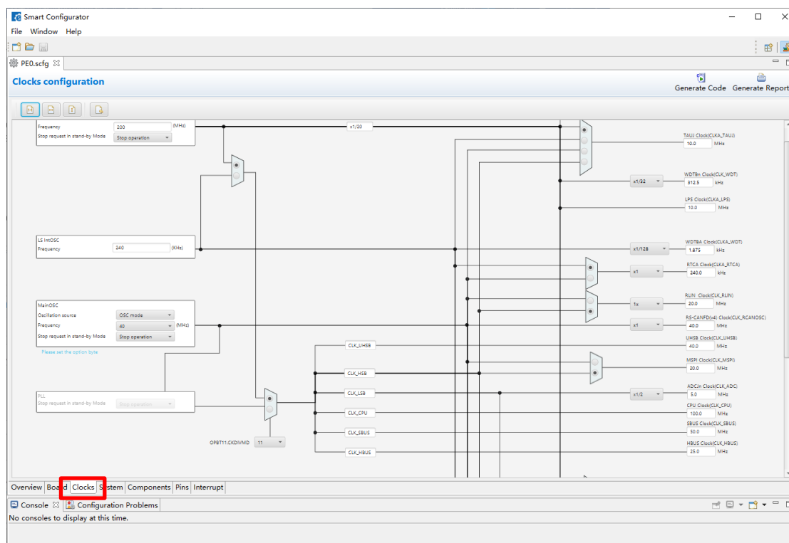
Figure 5-1. Configure clock
