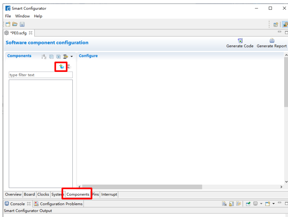
Figure 5-2. Add modules
