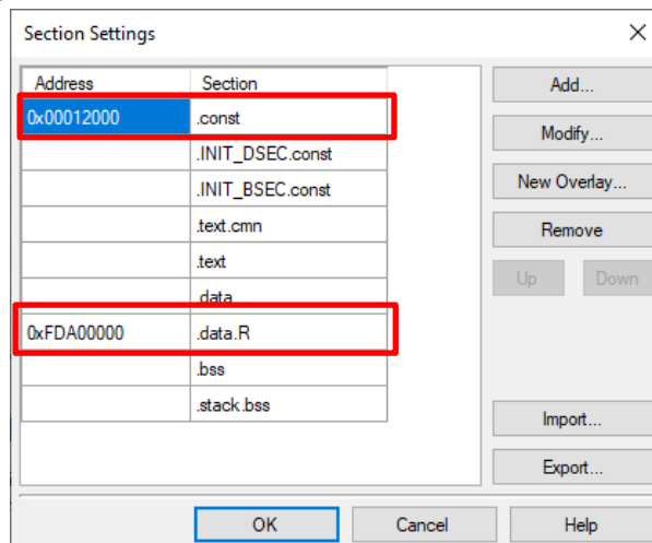
Figure 4-20. Setting in the subproject PE1
