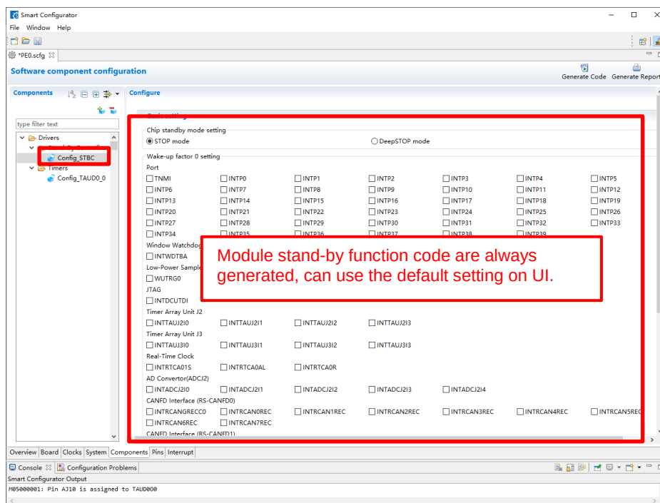
Figure 5-6. Add Stand-by Controller component
