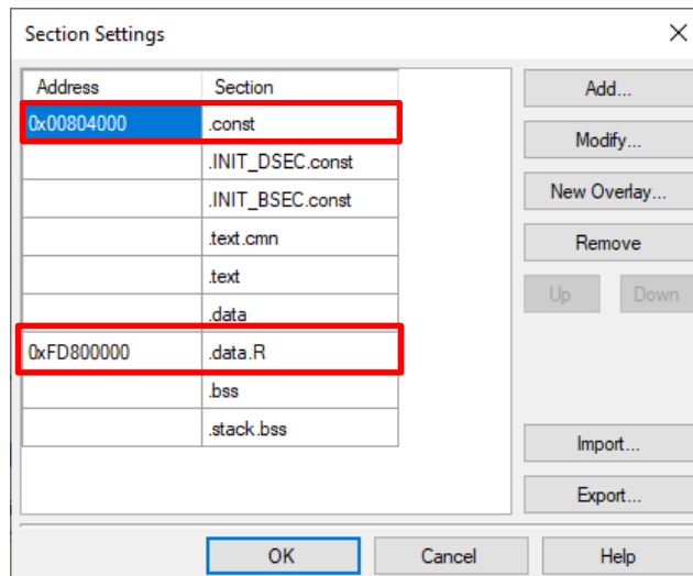
Figure 4-21. Setting in the subproject PE2
